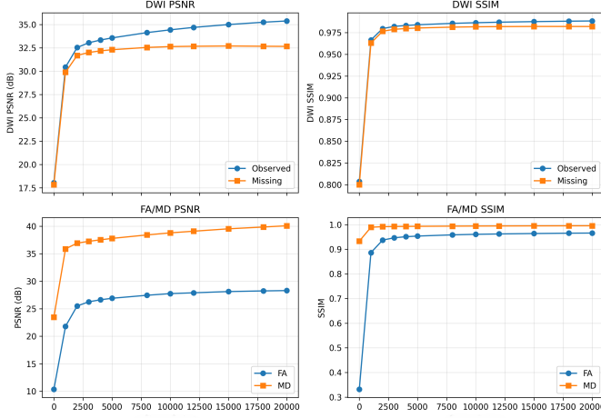
Fig. 8. Effect of optimization steps at b = 1000 s/mm 2 , R_k = 3 , with 15 observed directions.
