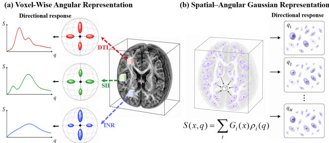
Fig. 1. Comparison of voxel-centered and primitive-centered spatial-angular dMRI representations. (a) A directional response is independently attached to each fixed voxel, (b) overlapping 3D Gaussian primitives provide shared spatial support and q-conditioned responses whose weighted aggregation yields the queried DWI signal.
