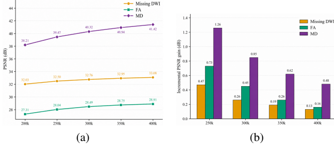
Fig. 9. Effect of the Gaussian primitive budget at b = 1000 s/mm 2 , R_k = 3 , with 15 observed directions. (a) DWI, FA, and MD PSNR, (b) incremental PSNR gains.
