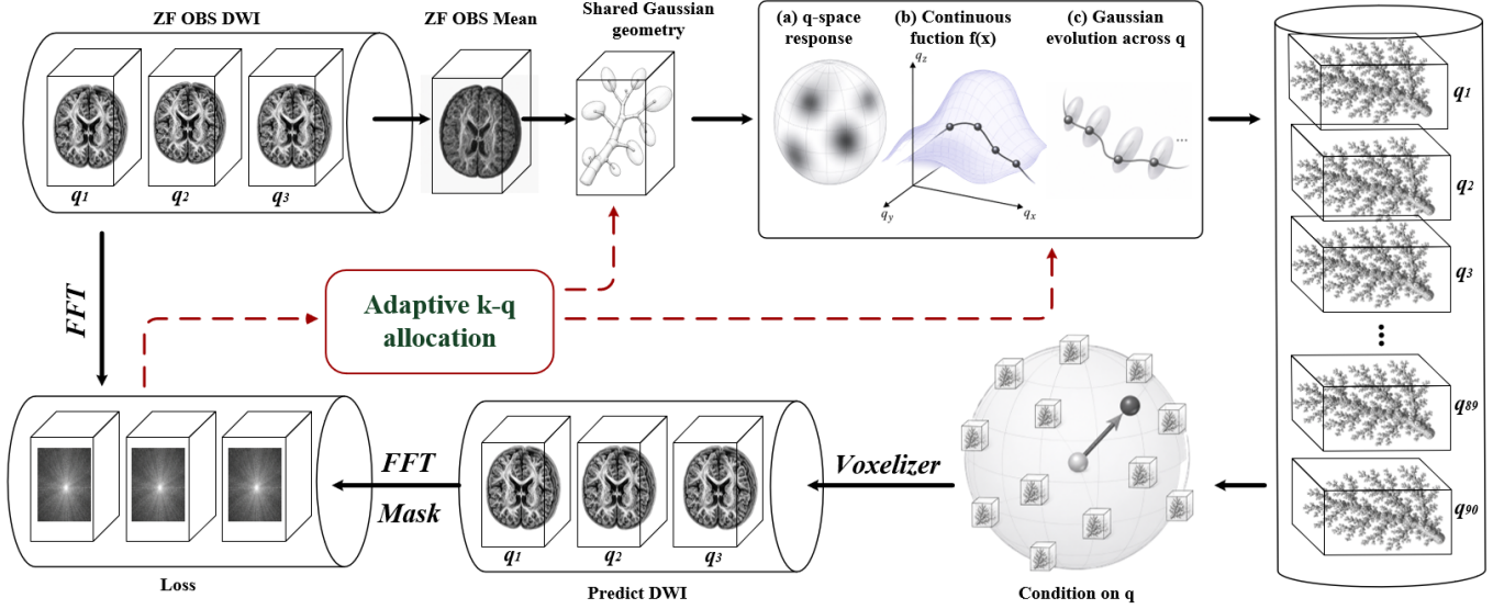
Fig. 2. Overview of the proposed diffusion-encoding spatial-angular Gaussian framework. A shared Gaussian scaffold with continuous tensor-residual responses is optimized using observed-direction reconstruction and sampled k-space consistency, while fitting residuals guide adaptive primitive allocation.
