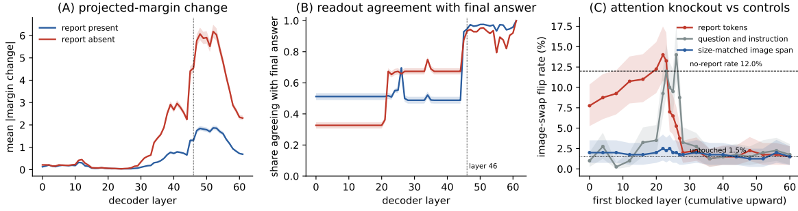
Figure 3. (A) Mean absolute change in the projected yes/no margin between the two images at each decoder layer, report present and absent, 44,786 trials, patient-clustered 95% intervals; the layer-61 values are the published 0.690 and 2.307. (B) Share of trials whose projected answer at each layer equals the final answer. (C) Report-token attention knockout, cumulative from the plotted layer upward, against the question-and-instruction span and a size-matched image span, 400 one-question cases.
