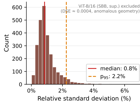
Figure 10: DSE estimation noise across 260 models and 10 datasets. Relative standard deviation of DSE across batches.
