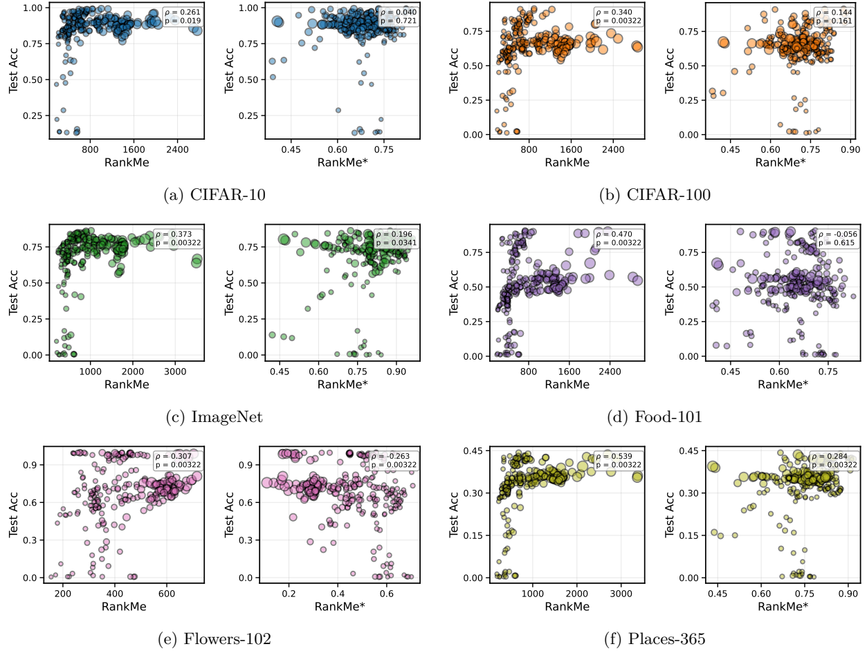
Figure 14: Comparison of RankMe and RankMe* against KNN probe test accuracy across six datasets. The \rho denotes the Spearman correlation and the corresponding p -value is annotated in each subplot. Marker size is proportional to each model’s representation dimensionality, scaled linearly relative to the highest-dimensional model.
