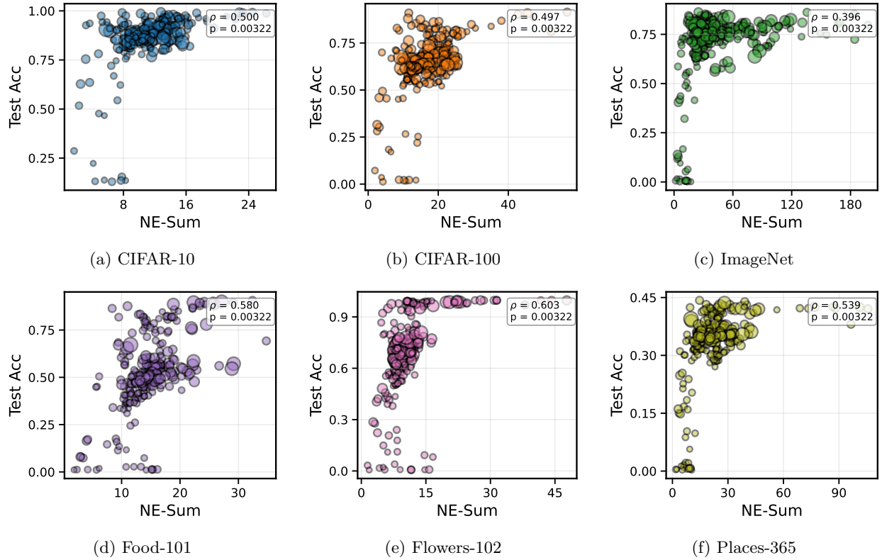
Figure 15: Comparison of NE Sum against KNN linear-probe test accuracy across six datasets. The \rho denotes the Spearman correlation and the corresponding p -value is annotated in each subplot. Marker size is proportional to each model’s representation dimensionality, scaled linearly relative to the highest-dimensional model.
