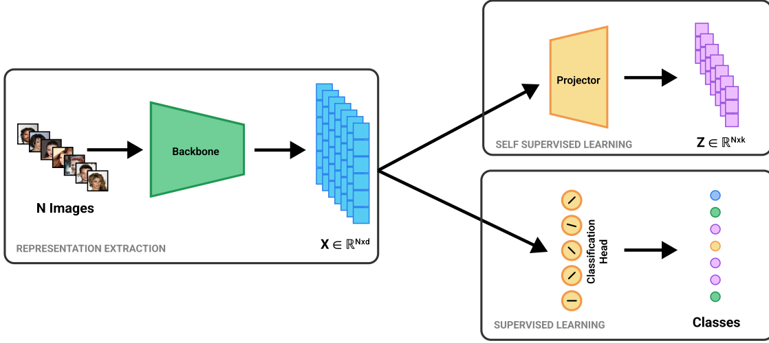
Figure 1: Illustration of the representation extraction pipeline for self-supervised (SSL) and supervised models. In SSL models, the projector MLP is discarded after training, and the backbone output X \in \mathbb{R}^{N \times d} is used as the representation. For supervised models, the penultimate layer activations are used as the representation, also denoted as X . In both cases, representation quality metrics are computed directly on X , without access to the projector embeddings Z or classification heads.
