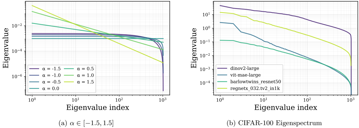
Figure 2: Comparison of real and synthetic eigenspectra in log-log scale. Real backbone representations with dimension d \in [1000, 1024] (Fig. 2b) exhibit spectral shapes consistent with the synthetically generated power-law family \lambda_i \propto i^{-\alpha} , \sum_{i=1}^d \lambda_i = 1 , under negative values of \alpha (Fig. 2a). This similarity justifies including \alpha < 0 in the synthetic sensitivity analysis
