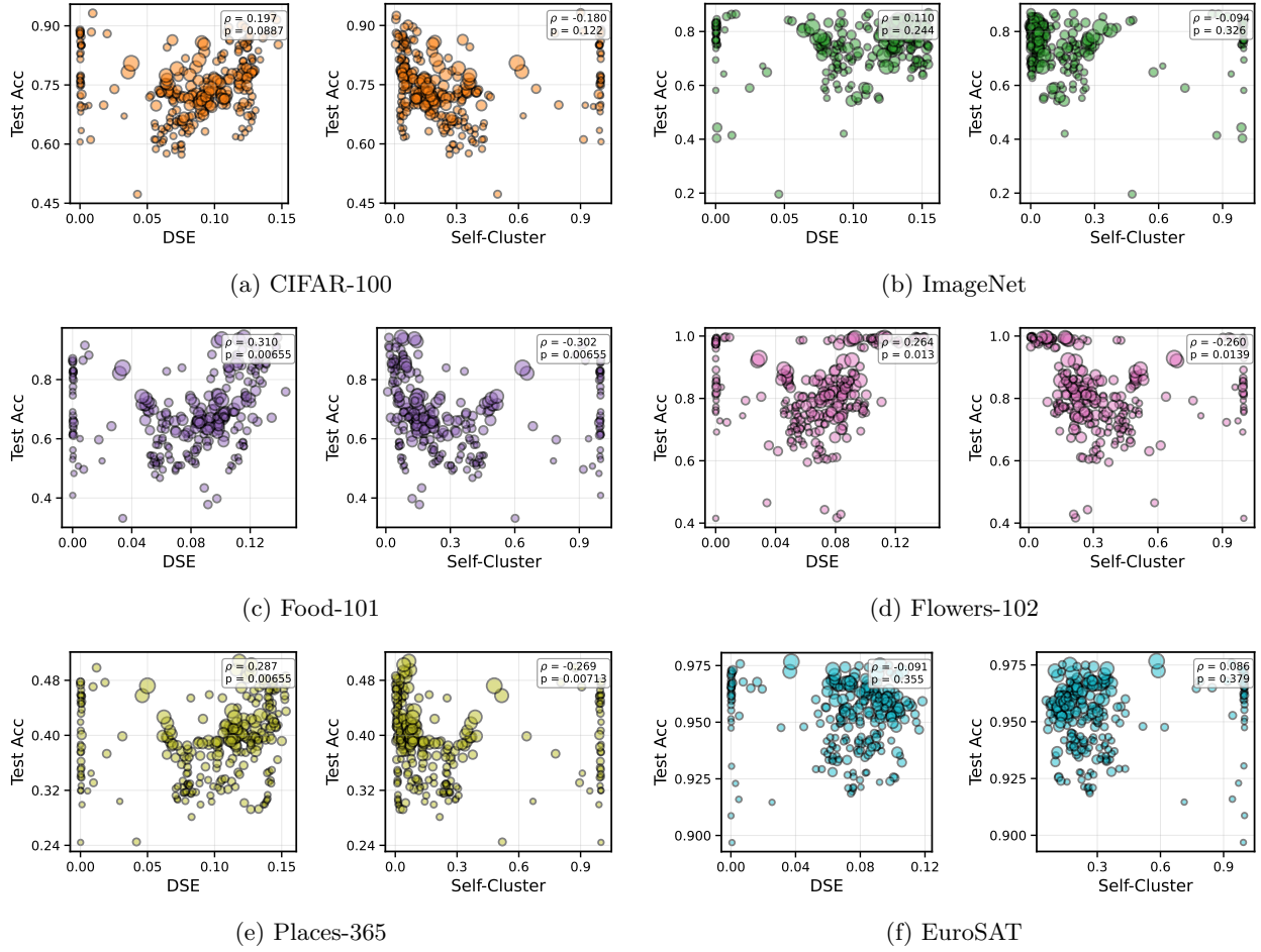
Figure 5: Comparison of DSE and Self-Cluster against OLS linear-probe test accuracy across six datasets. The \rho denotes the Spearman correlation and the corresponding p -value is annotated in each subplot. Marker size is proportional to each model’s representation dimensionality, scaled linearly relative to the highest-dimensional model.
