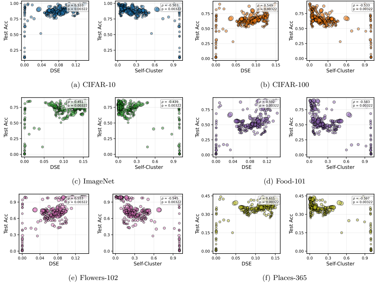
Figure 13: Comparison of DSE and Self-Cluster against KNN linear-probe test accuracy across six datasets. The \rho denotes the Spearman correlation and the corresponding p -value is annotated in each subplot. Marker size is proportional to each model’s representation dimensionality, scaled linearly relative to the highest-dimensional model.
