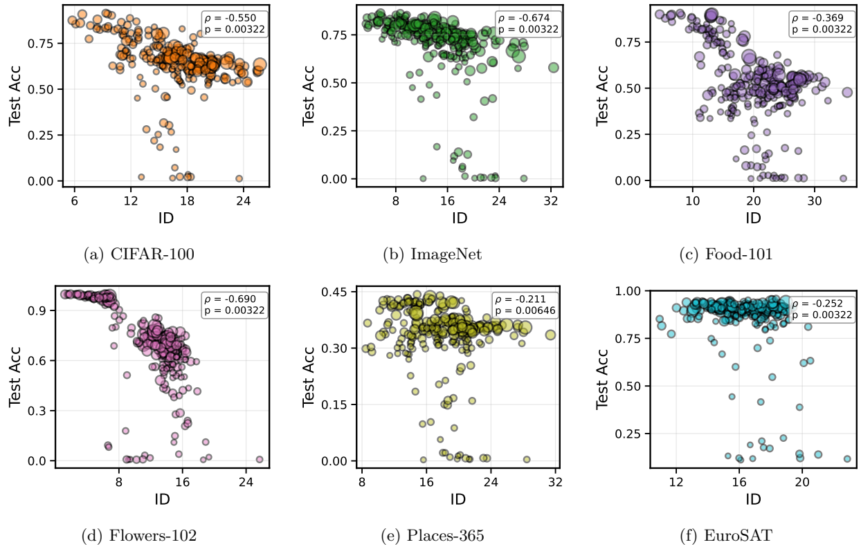
Figure 16: Comparison of ID against KNN probe test accuracy across six datasets. The \rho denotes the Spearman correlation and the corresponding p -value is annotated in each subplot. Marker size is proportional to each model's representation dimensionality, scaled linearly relative to the highest-dimensional model.
