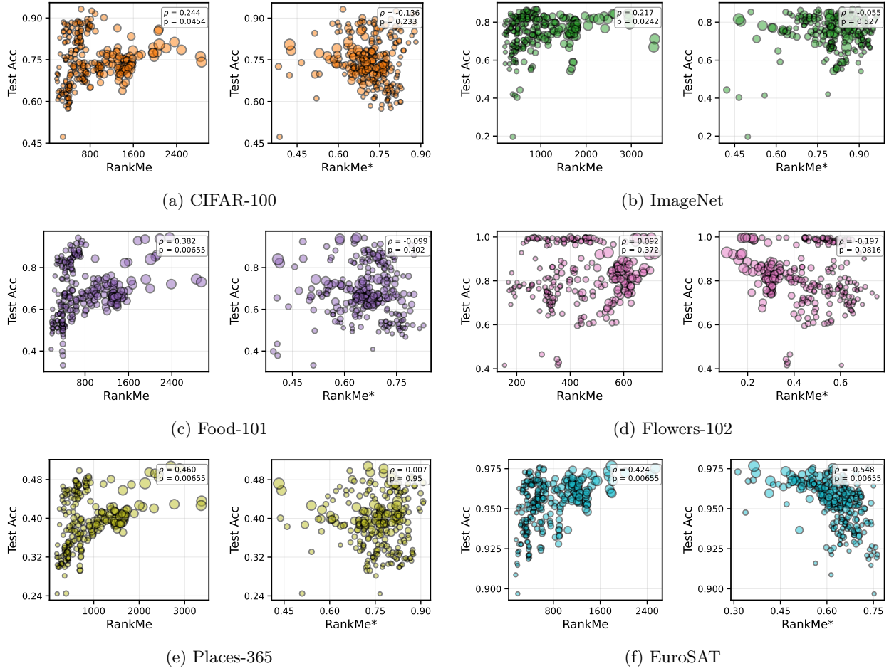
Figure 7: Comparison of RankMe and RankMe* against OLS linear-probe test accuracy across six datasets. The \rho denotes the Spearman correlation and the corresponding p -value is annotated in each subplot. Marker size is proportional to each model’s representation dimensionality, scaled linearly relative to the highest-dimensional model.
