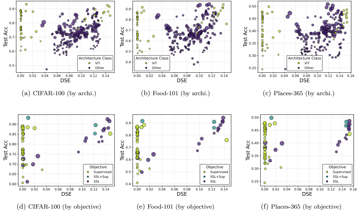
Figure 12: DSE metric values plotted against test accuracy across datasets. The top row shows all models coloured by architecture class, revealing that the models with extreme values predominantly belong to the ViT architecture class. The bottom row shows only ViT models coloured by training objective, illustrating that the near zero DSE values originate predominantly from Supervised and SSL+Sup models rather than SSL models. This suggests that the DSE metric may be a reliable predictor for SSL models (though the sample size is small), but is unreliable for Supervised and SSL+Sup models.
