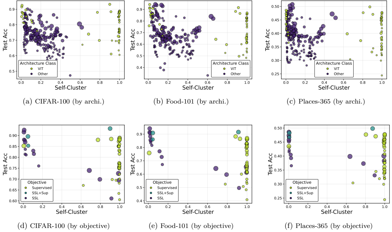
Figure 6: Self-Cluster metric values plotted against test accuracy across datasets. The top row shows all models coloured by architecture class, revealing that the models with extreme values predominantly belong to the ViT architecture class. The bottom row shows only ViT models coloured by training objective, illustrating that the near unit Self-Cluster values originate predominantly from Supervised and SSL+Sup models rather than SSL models. This suggests that the Self-Cluster metric may be a reliable predictor for SSL models (though the sample size is small), but is unreliable for Supervised and SSL+Sup models.
