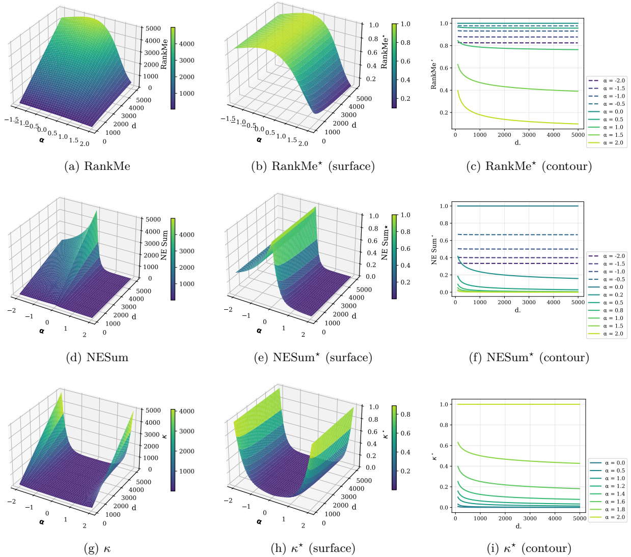
Figure 3: Sensitivity of spectral metrics RankMe, NE Sum, and \kappa to spectral shape ( \alpha ) and representation dimension ( d ), where eigenspectra are synthetically generated as \lambda_i \propto i^{-\alpha} with \sum_{i=1}^d \lambda_i = 1 . Each row shows the un-normalised metric (col. 1), the dimension-normalised surface (col. 2), and the normalised metric as a function of d for fixed values of \alpha (col. 3). Normalisation is performed by dividing by d , following the normalisation proposed in Tsitsulin et al. (2023) for RankMe, which we extend to all three metrics. In col. 3, dashed lines correspond to \alpha < 0 and solid lines to \alpha \geq 0 . Since \kappa is symmetric about \alpha = 0 (Fig. 3h), only \alpha \geq 0 is shown in Fig. 3i.
