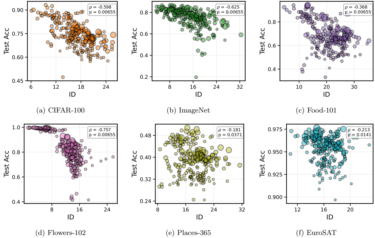
Figure 4: Comparison of ID against OLS probe test accuracy across six datasets. The \rho denotes the Spearman correlation and the corresponding p -value is annotated in each subplot. Marker size is proportional to each model’s representation dimensionality, scaled linearly relative to the highest-dimensional model.
