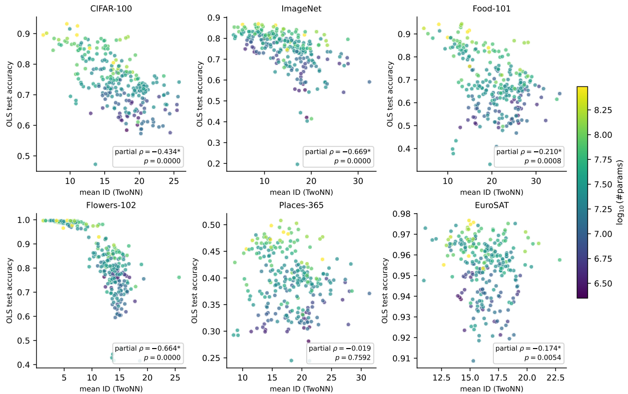
Figure 11: ID vs OLS test accuracy, coloured by \log_{10} parameter count, across six main datasets. Partial Spearman correlations controlling for log parameter count are annotated in each panel ( n = 255 ; 5 models excluded due to unavailable parameter counts). Asterisk (*) denotes p < 0.05 .
