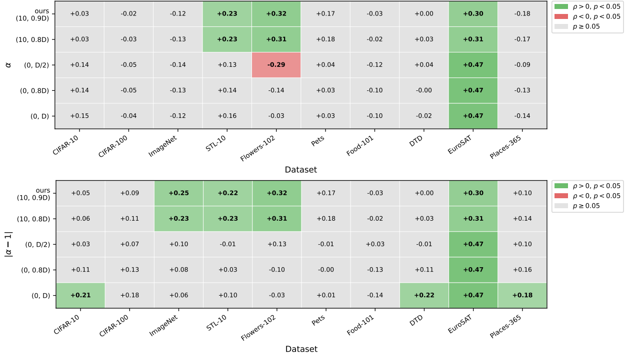
Figure 8: \alpha -ReQ fitting-range sensitivity. Spearman correlation between \alpha (top) and |\alpha - 1| (bottom) with OLS test accuracy, across five fitting ranges and ten datasets. Green: significant positive; red: significant negative; grey: p \geq 0.05 .
