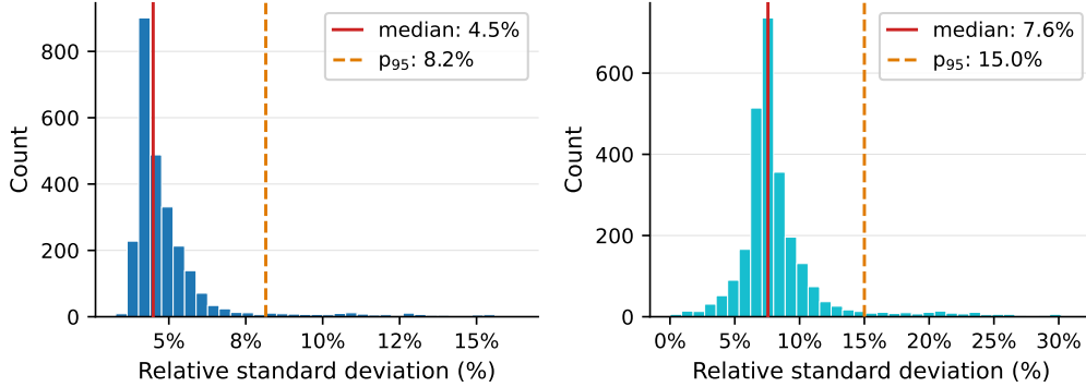
Figure 9: TwoNN intrinsic dimensionality (ID) estimation noise across 260 models and 10 datasets (2,600 model-dataset pairs). Left: Intra-batch subsample noise which is the relative standard deviation of ID across 20 within-batch subsamples (Number of repetition = 20, 90% subsampling rate within each batch). Right: Across-batch noise which is the relative standard deviation of the per-batch mean ID across batches. Median intra-batch and across-batch noise are 4.5% and 7.6% respectively, with 95th percentiles at 8.2% and 15.2%.
