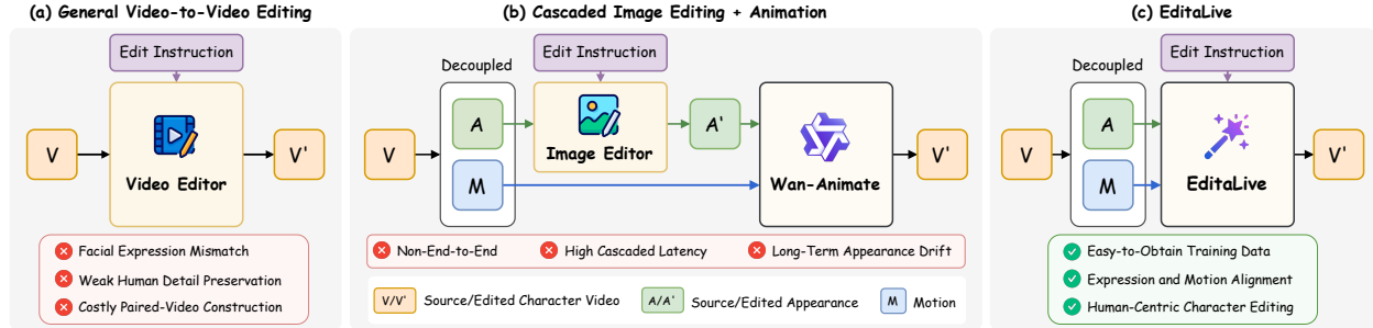
Figure 2 Comparison of three character video editing paradigms. (a) General Video-to-Video Editing directly transforms a source video V into an edited video V' , but often relies on costly synthetic video pairs that may contain facial-expression mismatches and weakened human details. (b) Cascaded image editing and animation first edits the source appearance A into A' and then animates it using motion M , introducing cascaded latency and potential long-term appearance drift. (c) EditaLive unifies appearance editing and motion-conditioned generation, learning from edited reference images and motion-aligned real videos to preserve facial expressions and body motion while enabling stable, low-latency streaming editing.
