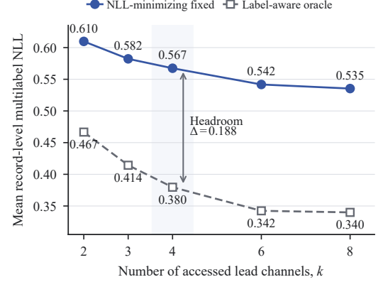
Fig. 1. Pre-holdout evidence for evaluator-conditioned channel-set heterogeneity. (A) The fold-10 controlled-evaluator NLL-minimizing fixed subset and the modal fold-9 k = 4 outputs of ECG-on-Demand and MGA. (B) Label-aware oracle first-channel choices across the fold-10 selection records; the six smaller shares are grouped as “Others.” (C) Fold-10 mean record-level multilabel NLL for the population-wide fixed subset and the label-aware per-record oracle. Oracle quantities are descriptive, controlled-evaluator- and NLL-specific, label-aware, and non-deployable.
