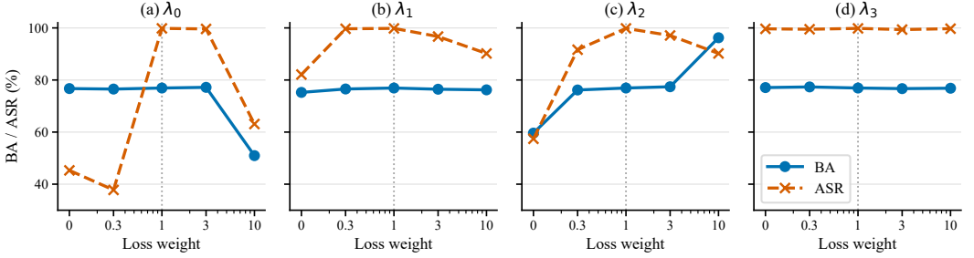
Fig. 7. Sensitivity to the four loss weights. Each panel varies one coefficient while fixing the other three to 1. Solid blue lines with circles denote BA, dashed orange lines with crosses denote ASR, and the vertical dotted line marks the default unit weight.
