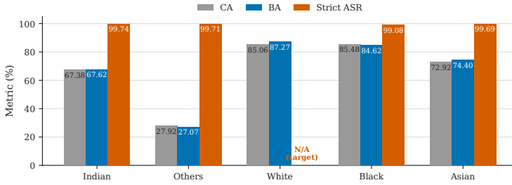
Fig. 9. Race-group analysis on UTKFace. Gray, blue, and orange bars denote CA, BA, and strict ASR, respectively. Strict ASR measures the proportion of triggered non-target samples classified as the target class. Since White is the attack target, its ASR is undefined and marked as N/A.
