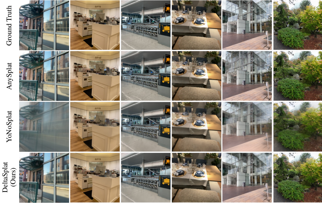
Figure 4: Qualitative results on DL3DV scenes.
