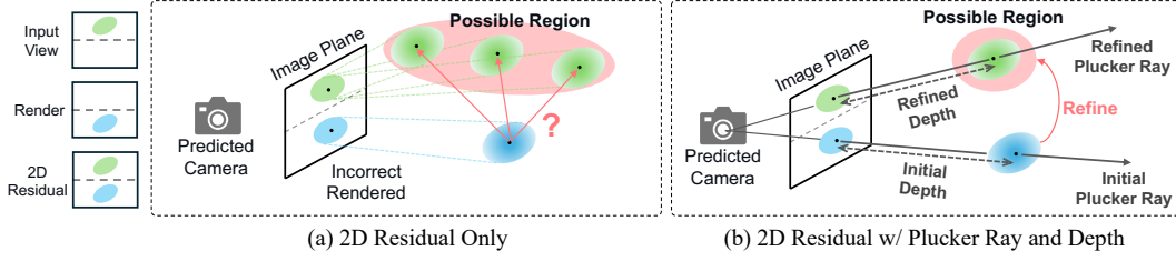
Figure 3: Geometry-guided residual encoding. (a) The 2D residual alone underdetermines the position update \Delta\mu : displacements along the viewing ray yield identical residuals, leaving a large possible region (red). (b) The per-pixel Plücker ray and rendered depth encode the line of sight and the current prediction’s position along it, a prior on the current geometry under which the possible region contracts.
