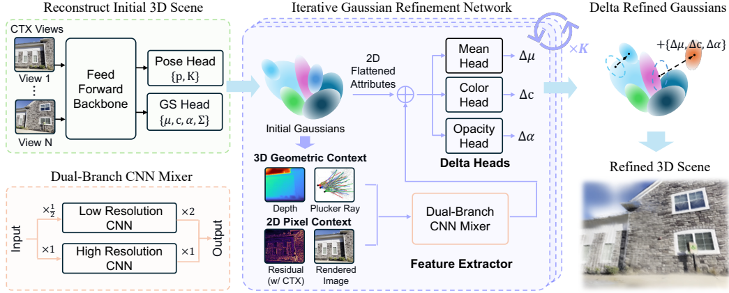
Figure 2: Method overview. The backbone predicts cameras and initial Gaussians; at each iteration, the refinement module encodes the render residual with the Plücker rays and the rendered depth, and decodes the per-Gaussian update \{\Delta\mu, \Delta c, \Delta\alpha\} , repeated K=3 times with shared weights.
