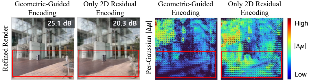
Figure 6: Effect of the 3D geometry prior. Each pair compares the geometry-aimed encoding with an encoding built from the 2D residual alone; the left pair shows the refined render and the right pair the per-Gaussian |\Delta\mu| . Without the Plücker-ray and depth channels the same residual drives larger and more scattered position updates, and PSNR falls from 25.1 to 20.3 dB.
