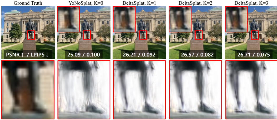
Figure 1: Iterative Gaussian refinement on a DL3DV scene in the pose-free setting. K denotes the number of refinement iterations applied. Starting from the feed-forward output of the YoNoSplat backbone ( K=0 ), each DeltaSplat iteration progressively recovers structures missing from the initial prediction: the statue’s legs, absent at K=0 , gradually emerge in both the rendered views (top, red box) and the underlying Gaussian geometry (bottom, with the ground-truth image crop as reference), with monotonic gains in PSNR and LPIPS.
