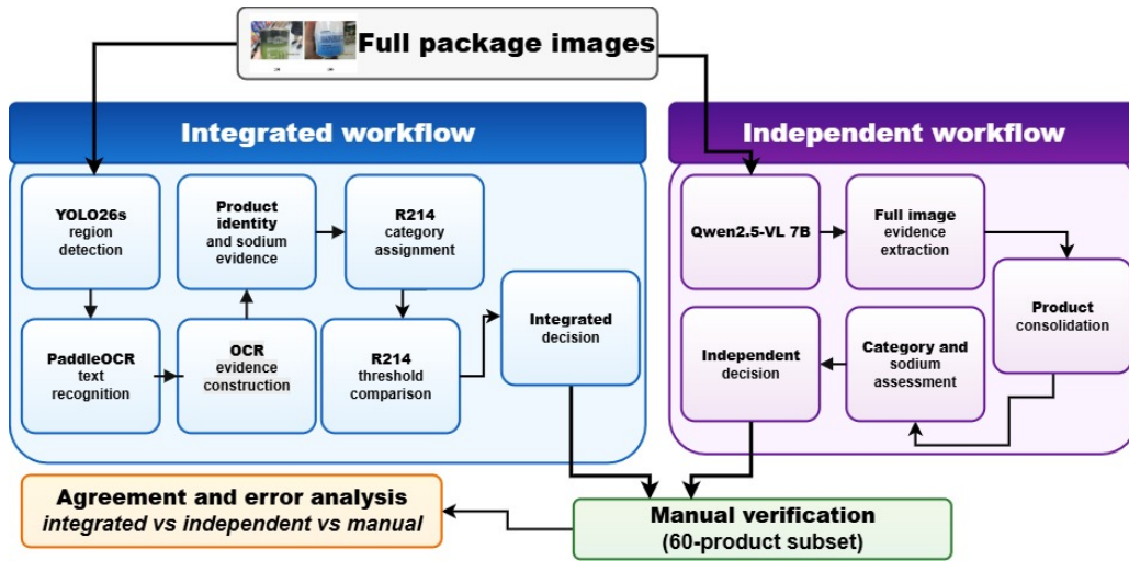
Fig. 1. Overview of the image-based R214 sodium screening and validation workflow. The integrated workflow produces product-level screening outcomes, the independent workflow provides a separate comparison, and manual verification checks a 60 product subset for agreement and error analysis.
