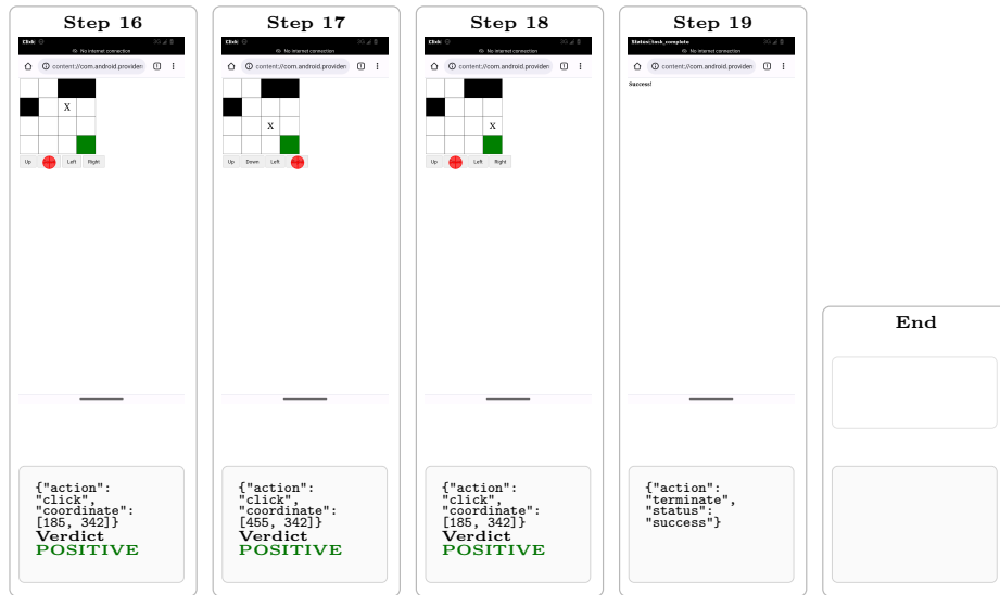
Fig. A3: AnchorGUI trajectory on BrowserMaze (continued), steps 16–19 and termination. Across the full episode, negative CSA records act as explicit correction anchors: they first redirect file opening from direct tap to Open with , and later help the policy recover from local maze-control mismatches instead of repeating them blindly.
