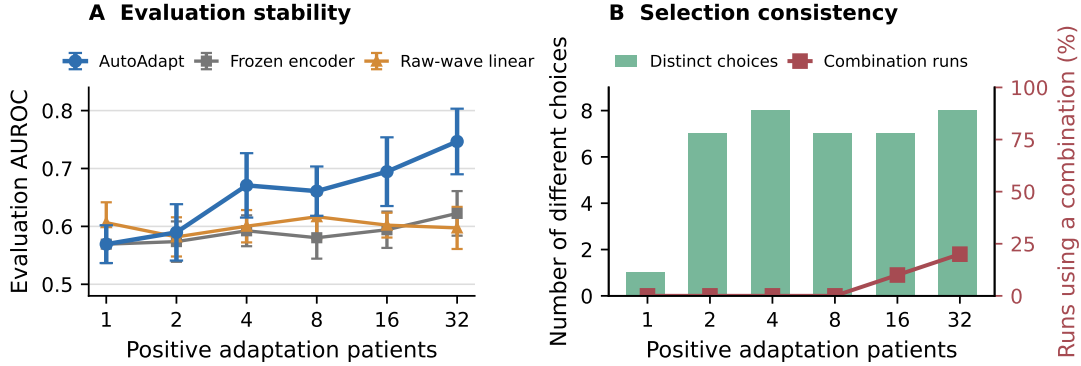
Figure 6: Stability on ALOTT new-pressor prediction as the adaptation panel grows from one to 32 positive patients, with an equal number of negative patients. Panel A reports evaluation AUROC over ten repeated panels against two fixed baselines. Panel B reports the number of distinct selections and the fraction using a recipe combination.
