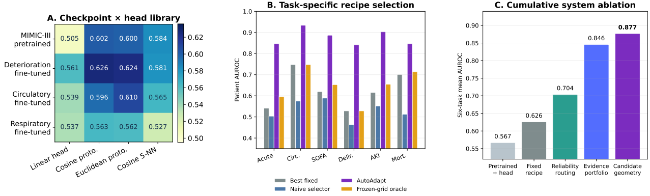
Figure 3: Checkpoint and recipe analysis on MIMIC-IV. Panel A tests source checkpoint and head pairings. Panel B compares a fixed recipe, naive adaptation-only selection, and the reliability-aware Automator. Panel C adds the Adapter and Automator components cumulatively.
