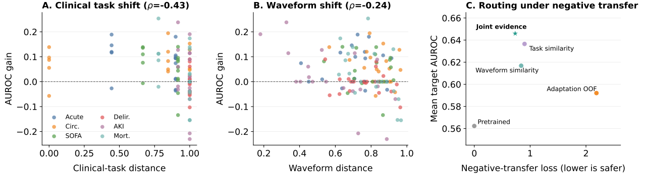
Figure 5: Checkpoint routing under distribution shift. Panels A and B show how transfer gain changes with task distance and waveform distance. Panel C compares routing rules. Every point uses the same target patients. Evaluation labels measure transfer gain but do not select a checkpoint.
