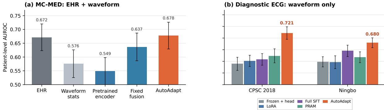
Figure 4: Cross-dataset comparisons. Panel A reports MC-MED macro AUROC over four tasks with sufficient patient support, comparing local EHR, waveform transfer, fixed fusion, and AUTOADAPT. Panel B reports macro AUROC over five shared diagnostic ECG tasks in CPSC and Ningbo. Methods use the same target folds within each dataset. The reference line marks chance AUROC.
