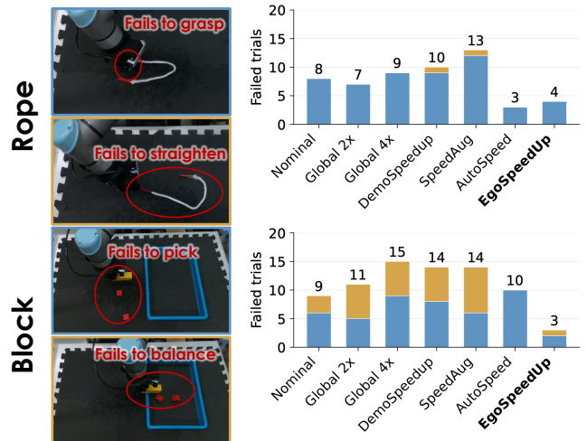
Fig. 5: Representative failure cases and phase-associated failure counts for Rope and Block. Rope failures are categorized as grasping and straightening, and Block failures as picking and unstable placement. Stacked bars report failed trials among 20 attempts per method and task; numbers above the bars indicate total failures. Failure counts are not normalized by the number of trials that reached each phase.
