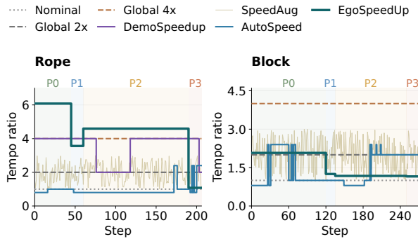
Fig. 4: Target tempo profiles for representative Rope and Block demonstrations. The horizontal axis denotes the original demonstration step, and the curves show the target tempo factor assigned to each training window. Global baselines use fixed tempo factors, whereas EgoSpeedUp assigns piecewise-constant target tempo factors derived from aligned human manipulation phases. The plotted values are training targets, not measured rollout speedups.
