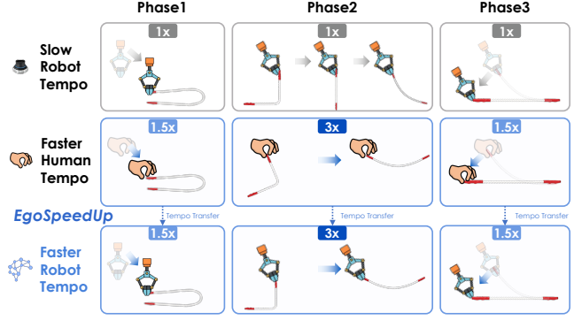
Fig. 1: EgoSpeedUp transfers phase-wise manipulation tempo from human to robot demonstrations. Human demonstrations implicitly encode task-appropriate manipulation tempo. For example, humans can efficiently straighten a rope by rapidly swinging it during the motion. EgoSpeedUp aligns slow robot demonstrations with this human tempo, enabling faster robot manipulation while maintaining task success.
