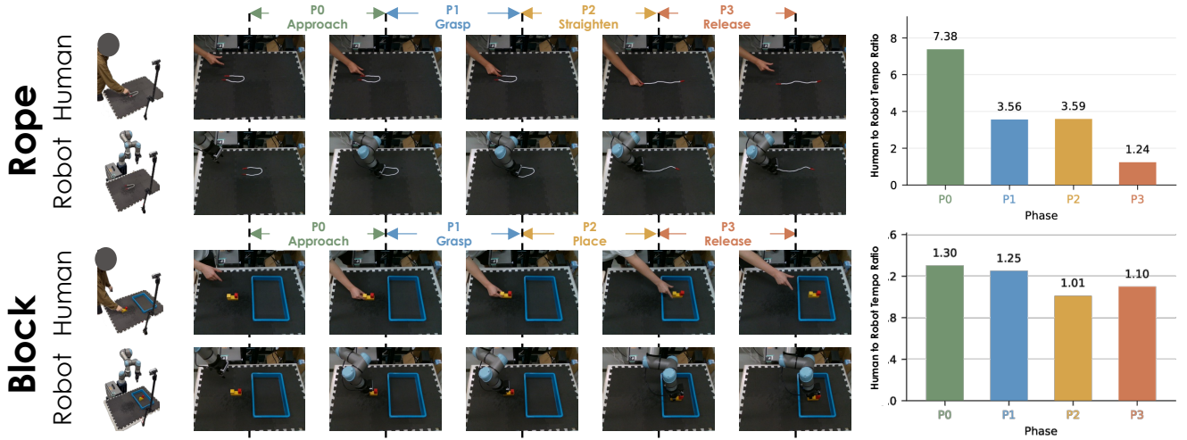
Fig. 3: Human–robot phase correspondence and phase-wise tempo ratios for the Rope and Block tasks. Representative human and robot demonstrations are aligned into four manipulation phases ( P0 – P3 ). The corresponding mean tempo ratios are computed from phase lengths and provide the temporal reference used by EgoSpeedUp.
