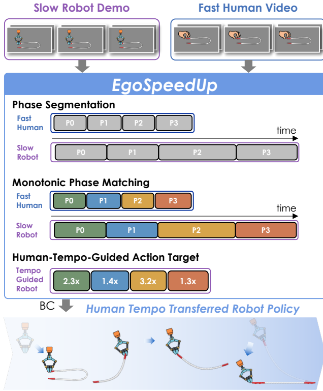
Fig. 2: Overview of EgoSpeedUp. Fast human videos and slow robot demonstrations are segmented into manipulation phases and aligned through monotonic phase matching. Corresponding phase lengths provide tempo ratios that determine phase-wise target tempos for the robot demonstrations. These tempos are used to retime future robot action targets, forming the EgoSpeedUp training data for behavior cloning.
