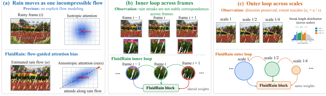
Figure 1: Physical motivation and Loop-in-Loop design of FluidRain. (a) Rain flow guides anisotropic attention. (b) Temporal persistence motivates the inner loop across frames. (c) Scale consistency motivates the outer loop across resolutions.
