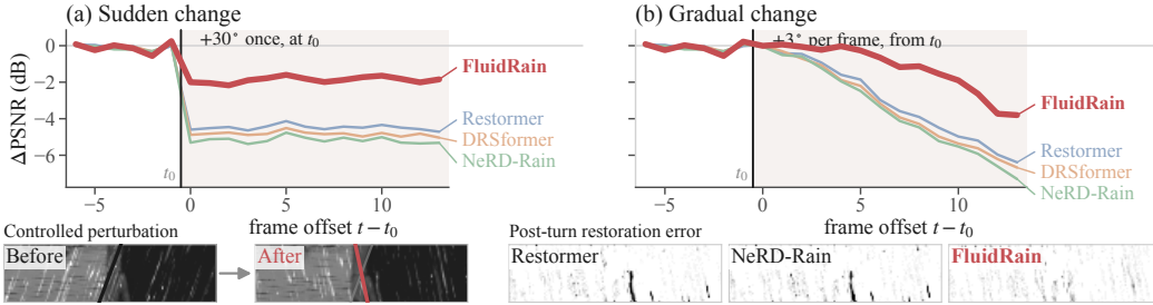
Figure 4: Robustness to changing rain motion on RainSyn-Gust. The bottom strip shows the controlled 30° perturbation and the corresponding post-turn restoration errors.
