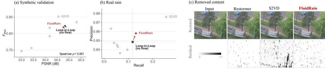
Figure 5: Evaluation of F_{\text{phys}} . (a) Correlation with PSNR on NTURain. (b) Precision–recall on real rain. (c) Restored crops and residuals.
