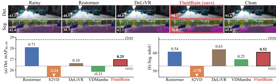
Figure 6: Downstream perception under rain.
