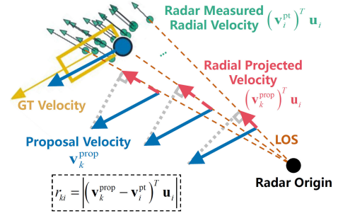
Fig. 4: Doppler-consistency geometry in PGCA. The 2D query velocity proposal \mathbf{v}_k^{\text{prop}} and the ego-compensated point velocity \mathbf{v}_i^{\text{pt}} are projected onto \mathbf{u}_i , the unit LOS direction from the source radar to point i at its measurement timestamp. All vectors are expressed in the reference frame. The absolute difference between their signed LOS projections defines the residual r_{ki} used in cross-attention.
