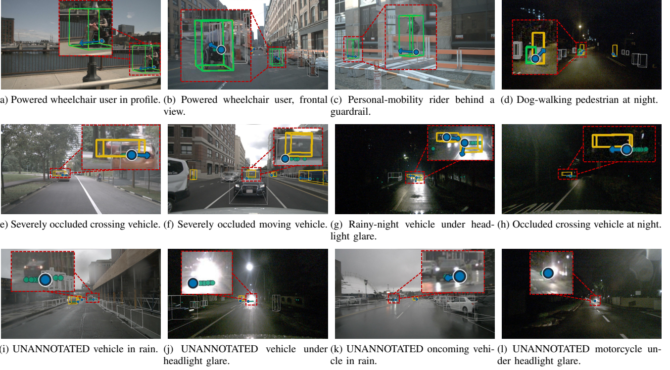
Fig. 1: Qualitative results of PART in rare-object, adverse-condition, and incomplete-annotation cases. Bright-green, yellow, and gray boxes denote special-category moving objects excluded from the standard nuScenes evaluation, moving ground truth used in our evaluation, and other annotated objects, respectively. Teal markers show moving radar returns; blue markers and arrows show PART predicted surface points and ground-plane velocities, respectively. (a)–(d) present rare and safety-relevant objects; (e)–(h) cover occlusion, low illumination, rain, and headlight glare; and (i)–(l) show moving objects unannotated in nuScenes. These examples illustrate PART’s behavior across rare objects, adverse conditions, and incomplete annotations.
