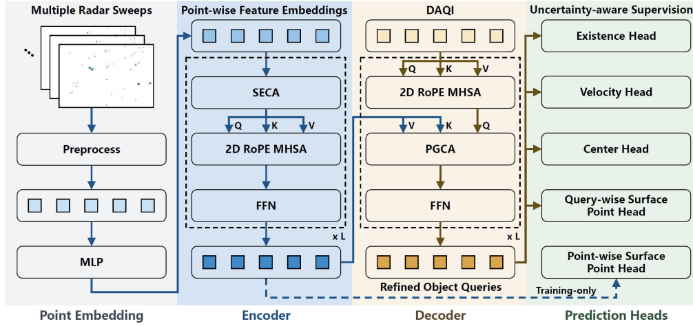
Fig. 2: Overview of the proposed PART. Blue paths encode radar points, while gold paths initialize and refine DAQI queries.
