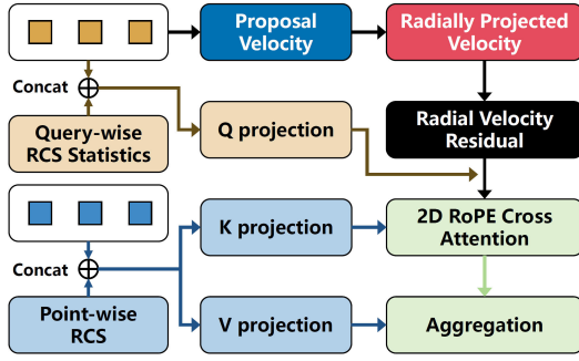
Fig. 3: Detailed architecture of PGCA.
