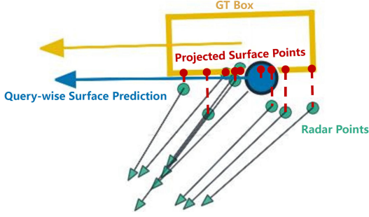
Fig. 5: Surface-point targets are obtained by projecting radar points and query references onto the nearest location on the ground-truth box perimeter.
