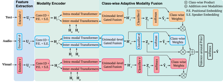
Fig. 2: Method overview. Building on SDT [21], unimodal features \mathbf{U} are projected into \mathbf{H} and processed by intra- and inter-modal Transformers to obtain enhanced representations \mathbf{H}' . We introduce class-wise adaptive modality fusion and a valence-arousal prior that biases the final prediction \hat{\mathbf{Y}} toward plausible affective transitions.
