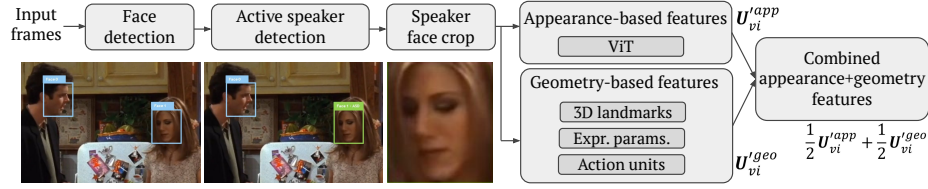
Fig. 3: Overview of the visual feature extraction. Speaker face crops are obtained from T = 16 frames per utterance, then encoded as a combined representation of appearance- and geometric-based facial features before entering the visual modality encoding stage.
