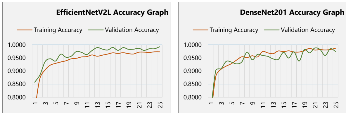
Figure 5. Training and Validation Accuracy Graph for the Top 4 Baseline Models
