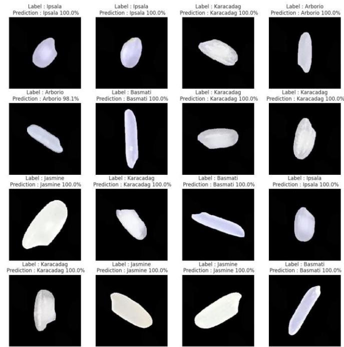
Figure 11. Example Test Result for Externa Data Validation
