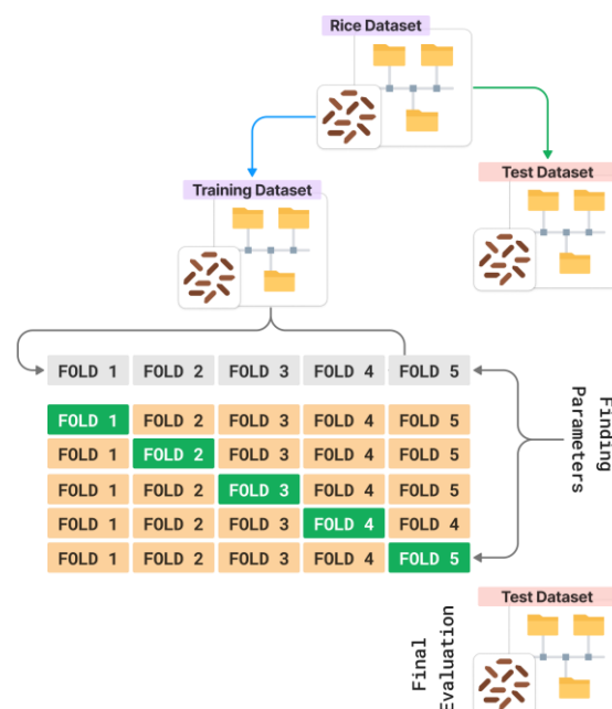
Figure 8. 5-Fold Cross-Validation Method
