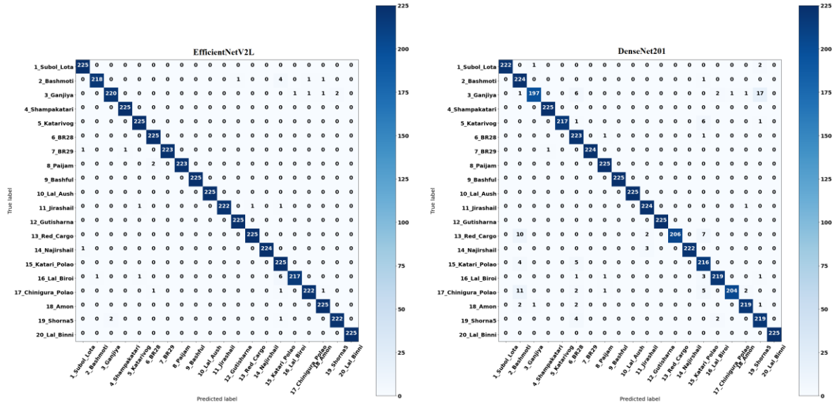
Figure 7. Confusion Matrix for the Top 4 Baseline Models
