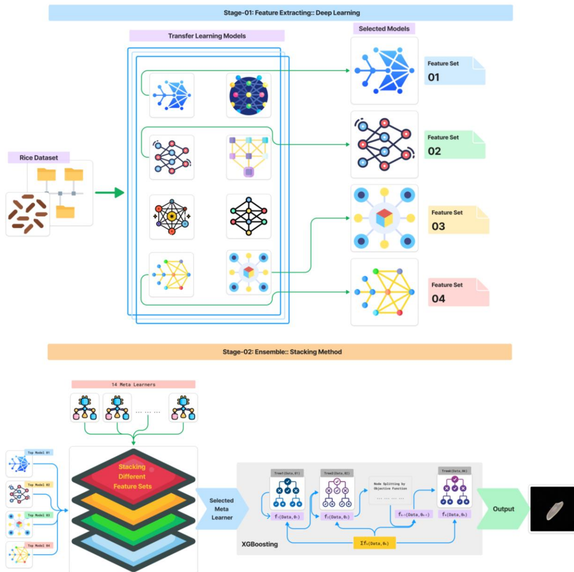
Figure 3. Proposed Ensemble Model Architecture
