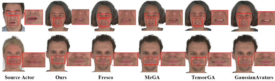
Figure 3: Qualitative comparison on cross-reenactment of head avatars. Our results show cleaner lip boundaries and more coherent mouth structures under cross-identity expression transfer.
