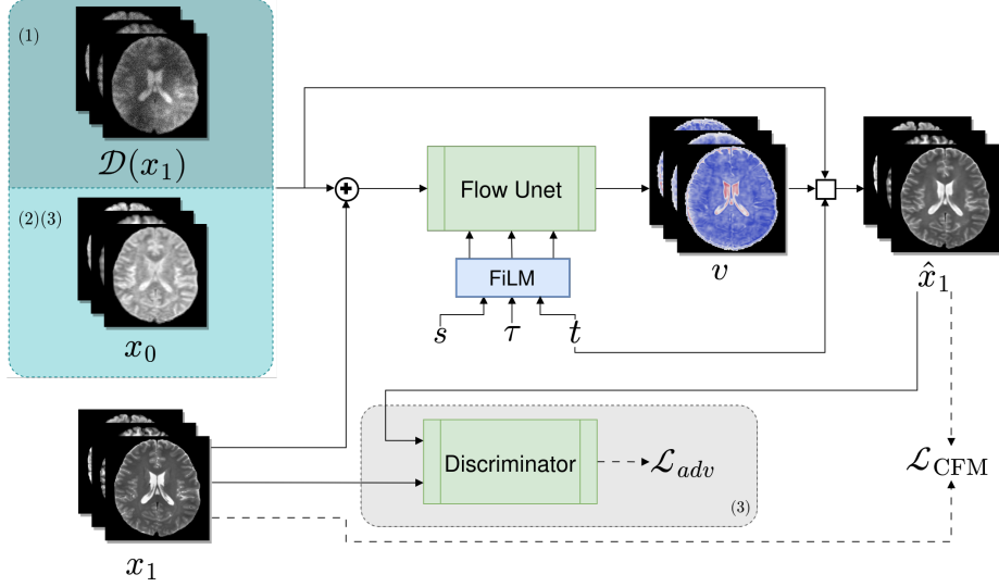
Fig. 1. The overall training architecture. Training is split into three stages, shown here as (1), (2), (3). In the pretraining stage the source ( x_0 ) is a degraded copy of the target ( x_1 ), since this cohort is unpaired; the network learns to restore it. In the second and third stages we continue with paired training. In the third stage, adversarial refinement, a discriminator judges the outputs of our CFM model and supplies an adversarial loss. The source field s , target field \tau , and the timestep t are embedded and injected through FiLM. During training the network predicts a velocity that transports the source towards the target; at inference this velocity is integrated over several steps.
