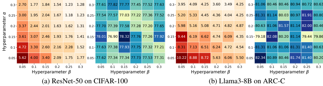
Figure 8: Sensitivity to \alpha and \beta of EUA-Cal. ECE ( \downarrow ) is shown in warmer colors, and ACC ( \uparrow ) is shown in cooler colors.
