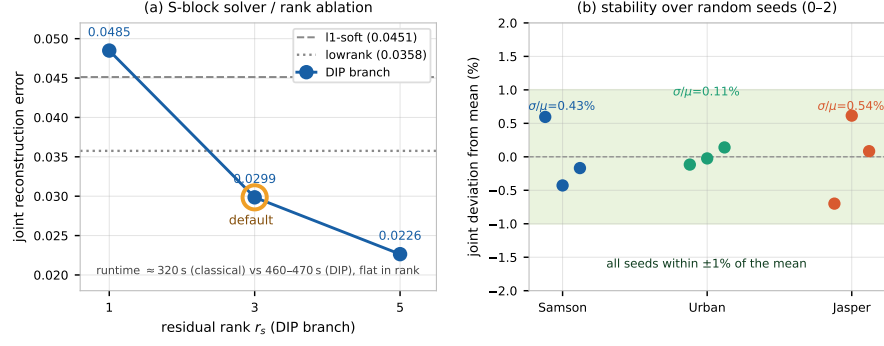
Fig. 3. (a) S-block solver/rank ablation on Urban under the fixed N-FINDR prior: joint error versus residual rank for the DIP branch, with non-DIP 11-soft and low-rank S-blocks shown as references. (b) stability of the joint error over three random DIP seeds; all runs stay within \pm 1\% of the per-dataset mean.
