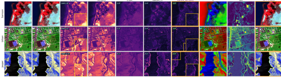
Fig. 4. S-block residual suppression on Samson, Urban, and Jasper under the fixed N-FINDR prior. Columns show the input image, \mathbf{A}\mathbf{X} , the input/captured/final residuals for the different S-blocks (11-soft, lowrank_r3, lowrank_dip), abundance \mathbf{X} , drift |\Delta\mathbf{X}| , and restored \mathbf{A}\mathbf{X} + \mathbf{S} . Residual maps share a per-row scale; badges report reconstruction SAM.
