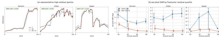
Fig. 5. Spectral evidence of residual refinement. (a) for one high-residual pixel per dataset, \mathbf{A}\mathbf{X} + \mathbf{S} better matches \mathbf{Y} and reduces per-pixel SAM. (b) across all pixels grouped by fixed-prior residual quartiles, \mathbf{S} consistently lowers the median SAM, with larger gains in higher-residual regions.
