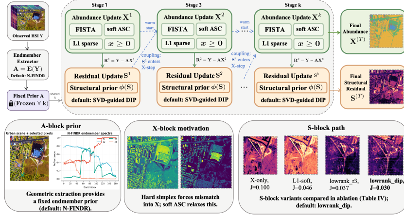
Fig. 1. Overview of the proposed interpretable stage-wise hyperspectral unmixing framework (I-HyperSU). The A-block provides a frozen endmember prior, the X-block performs abundance estimation with soft relaxation, and the S-block captures structured mismatch through progressive residual refinement.
