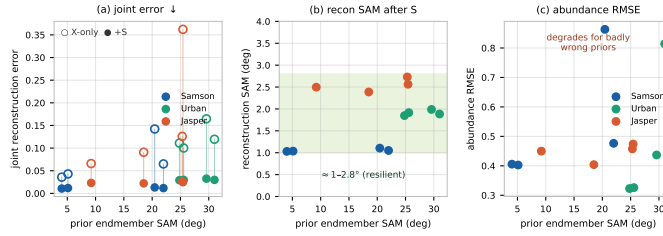
Fig. 7. Prior-mismatch stress test over four extractors (N-FINDR, VCA, ATGP, FIPPI) on the three datasets. (a) X-only joint error (○) grows with prior SAM while joint error with S (●) stays low. (b) reconstruction SAM after S stays low across extractors. (c) abundance RMSE instead degrades for badly wrong priors.
