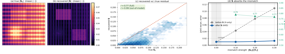
Fig. 6. Synthetic validation with a known non-negative residual \mathbf{S}_0 (stray-light/haze + striping; rank 5; partly out of \text{span}(\mathbf{A}) ; true endmembers fixed). (a,b) true |\mathbf{S}_0| vs. recovered |\mathbf{S}| (strength 0.20). (c) recovered vs. true residual. (d) joint error before vs. after \mathbf{S} across mismatch strengths, with \text{corr}(\mathbf{S}, \mathbf{S}_0) and the \mathbf{S}_0=0 control.
