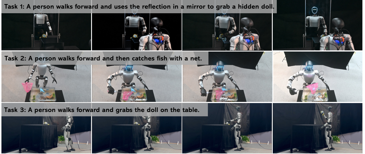
Figure 5: Representative real-world execution sequences. Rows show the three evaluated tasks, from top to bottom: Walk to Mirror (W2M) , approaching the table and grasping a hidden doll using mirror observations; Walk to Fish (W2F) , approaching the tank and scooping a toy fish with a handheld net; and Walk to Doll (W2D) , approaching the table and grasping a directly visible doll.
