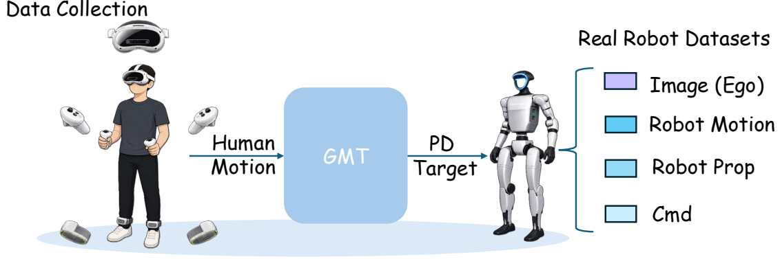
Figure 4: Overview of the data collection system. During the data collection stage, an operator uses a VR-based teleoperation system to generate low-level motion commands, and a pretrained whole-body motion tracker controls the humanoid robot. We record synchronized real-world trajectories comprising egocentric images, proprioceptive observations, and motion commands.
