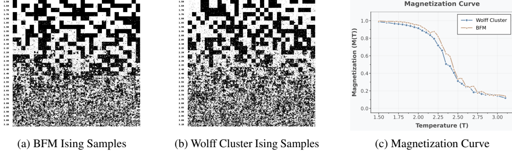
Figure 10: Comprehensive evaluation of Ising model generation across the continuous temperature spectrum (1.50 to 3.10). (a) and (b) show the visual evolution of spin lattices generated by BFM and the ground-truth Wolff cluster [33] algorithm, respectively. (c) Quantitative comparison of the absolute magnetization M(T) , demonstrating that BFM accurately captures the thermodynamic properties.
