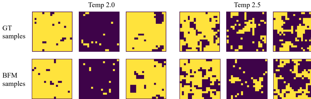
Figure 9: Comparison of 20 \times 20 Ising lattice samples generated by BFM and ground-truth samples at temperatures 2.0 and 2.5.
