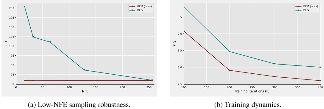
Figure 1: Comparison of BFM and BLD under reduced inference steps and during training. (a) FID versus NFE on LSUN Churches ( 256 \times 256 ), evaluated from the 100K-iteration checkpoints trained with 256 sampling steps using the linear probability path scheduler, where only the inference NFE is varied. (b) Training convergence comparison on LSUN Bedrooms ( 256 \times 256 ). We visualize the FID scores from 100K to 400K training iterations ( \times 10^3 ). Both BFM and BLD are trained under identical experimental settings using a linear scheduler. BFM reaches lower FID consistently throughout this range.
