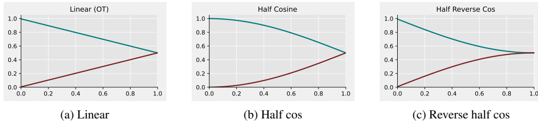
Figure 5: Bernoulli probability path schedulers.
