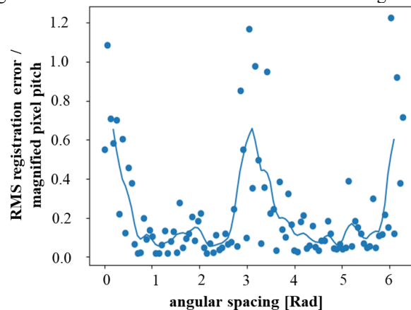
Figure 5: RMS registration error, normalized by the magnified detector-pixel size, when adding a second view at different angular separations using stochastic grid-search optimization with FF-35 radiograms.
