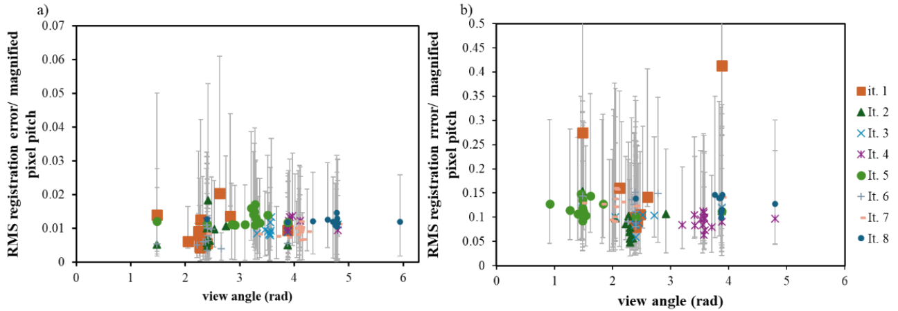
Figure 6: Greedy view-angle optimization using simulated target images (a) without noise and (b) with Gaussian noise. Each point summarizes eight registrations initialized with randomly directed pose perturbations; error bars denote standard deviations.
