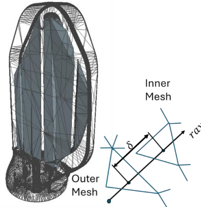
Figure 3: Schematic of the thickness measurement. A ray is cast from a known point fixed relative to the exterior mesh, and thickness is measured between its first intersections with the exterior and interior meshes.
