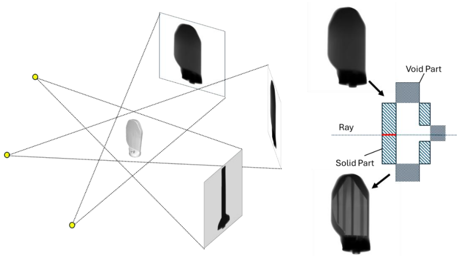
Figure 1: Schematic of simulated-radiogram generation. Rays originate from a point source, form a cone beam, and pass through the center of each detector pixel. Internal voids are handled by combining overlapping solid and void depth maps and calculating the path length through solid material while excluding the path through voids (red).
