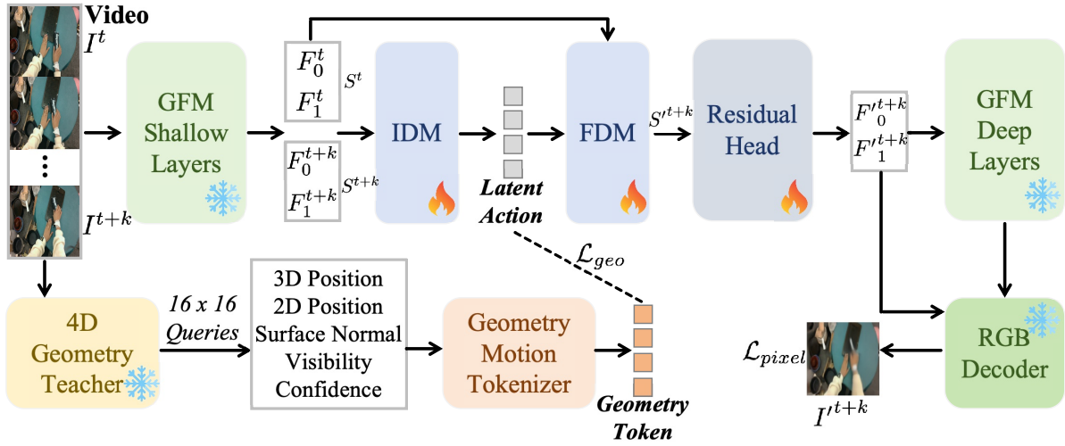
Fig. 1: Overview of GeoLAM. Frozen shallow GFM features encode the two video endpoints. The inverse dynamics model (IDM) compresses their transition into latent-action tokens, and the forward dynamics model (FDM) predicts future features from the current state and these tokens. Frozen deep GFM layers and an RGB decoder provide the reconstruction objective \mathcal{L}_{\text{pixel}} . During training, a frozen 4D teacher converts reliable 3D/2D motion and surface-normal changes into geometry-motion targets for \mathcal{L}_{\text{geo}} . Snowflakes and flames denote frozen and trainable modules, respectively.
