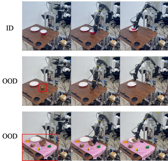
Fig. 4: Real-world bowl-placement task on Agilex Piper. Representative executions of our policy, with time progressing from left to right. From top to bottom: the in-domain (ID) setting, an out-of-distribution (OOD) bowl, and an OOD scene with a different tabletop covering and additional distractors. Red boxes highlight the object and scene changes.
