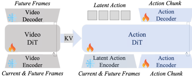
Fig. 2: Geometry-grounded latent actions for the world action model: during training, a frozen encoder supplies continuous transition targets and future-video prediction regularizes the Video DiT, whereas inference jointly denoises latent actions and action chunks using only cached current-observation key-value features. Snowflakes and flames denote frozen and trainable modules, respectively.
