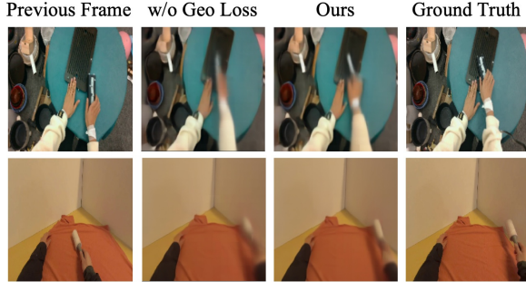
Fig. 6: Qualitative effect of 4D geometric supervision. Each row shows a human-video transition. From left to right: the previous frame, reconstruction without D4RT supervision ( \mathcal{L}_{\text{pixel}} only), full GeoLAM reconstruction, and the ground-truth future frame. Geometry supervision reduces smearing around moving hands and tools and better preserves their outlines.
