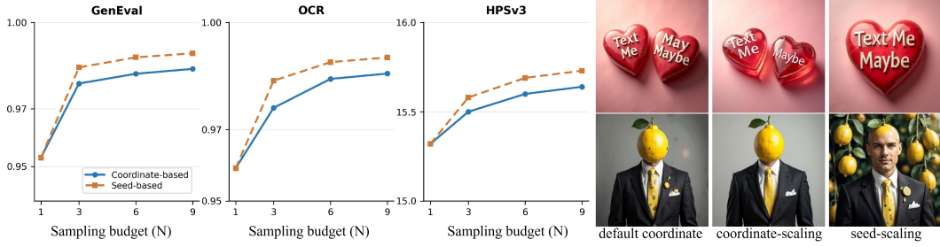
Figure 5: Demonstration of coordinate-based and seed-based test-time scaling.
