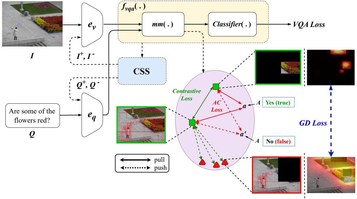
Figure 1: An overview of our training framework. The VQA baseline and CSS module generate feature triplets (z, z^+, z^-) , optimized via a three-stage curriculum that progressively introduces our Batch-Contrastive ( \mathcal{L}_{BC} ), Answer-Contrastive ( \mathcal{L}_{AC} ), and Gradient-Discrepancy ( \mathcal{L}_{GD} ) losses.
