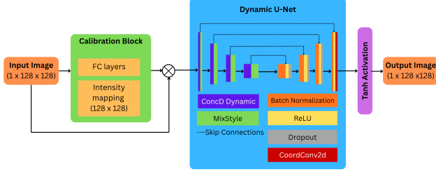
Fig. 1. DE-GAN generator. A voxel-calibration block precedes a U-Net encoder-decoder with dynamic convolution, MixStyle, dropout, and CoordConv. Skip connections retain local anatomy while the output head synthesizes enhanced FLAIR intensity.
