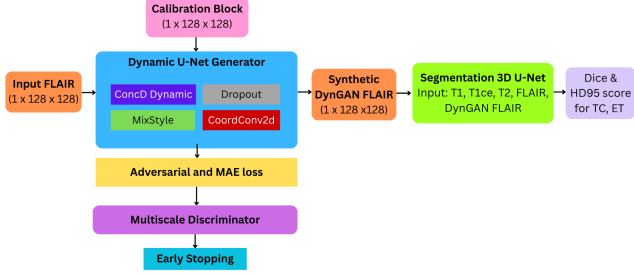
Fig. 2. DE-GAN applies voxel calibration and a dynamic U-Net generator to produce enhanced FLAIR slices. A two-scale discriminator evaluates real and synthetic pairs; the enhanced output is then fused with the original MR modalities for 3D segmentation.
