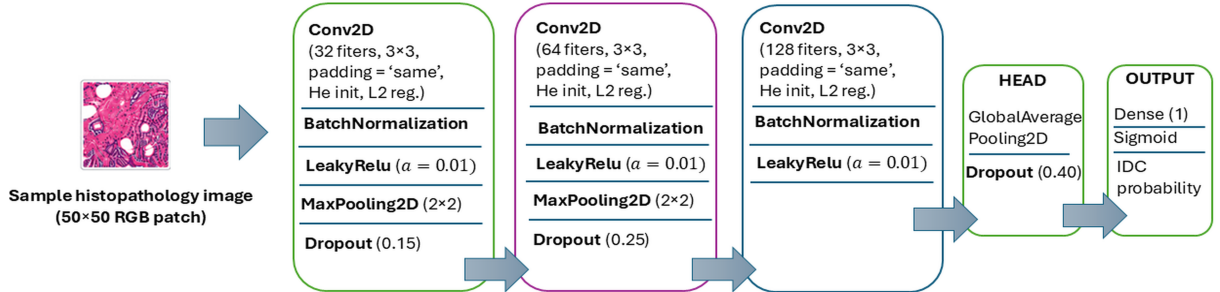
Fig. 2 CNN architecture used for IDC patch classification and shared across all distributed learning protocols
