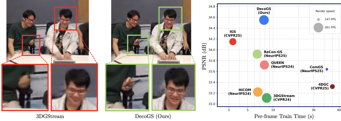
Figure 1. Quality and efficiency comparison. DecoGS achieves superior reconstruction quality while maintaining efficient streaming performance. The left images illustrate high-fidelity rendering results produced by DecoGS in dynamic regions. The right plot compares DecoGS with prior streaming methods [11, 17, 18, 20, 24, 55, 72] demonstrating the effectiveness of static–dynamic decoupling.
