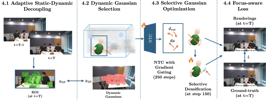
Figure 2. Overview of DecoGS. Given a set of multi-view video streams, DecoGS reconstructs an FVV stream of the dynamic scene. At t = 0 , we optimize a set of initial 3D Gaussians, and for each t > 0 , we compute a pixel-wise difference mask to isolate dynamic regions, dilated via max-pooling to capture motion boundaries. Throughout training, we optimize the NTC for 250 steps to rotate and translate Gaussians from the previous timestep t = T - 1 . At step 150, we employ selective densification that limits the spawning of Gaussians only to the selected areas, enabling the emergence of new objects. From this step onward, we optimize the selected Gaussians jointly with NTC using a focus-aware loss that concentrates the optimization to the detected ROI.
