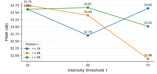
Figure 5. Sensitivity of Stage 2 PSNR to intensity threshold \tau and dilation radius r on the discussion scene. DecoGS is robust around \tau=25 , r=48 (our default).
