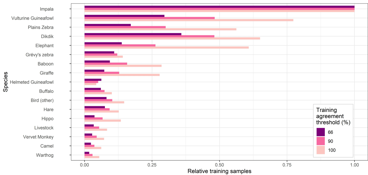
Figure S2: Relative number of training samples for the unbalanced Prickly Project Kenya dataset; number of samples for each class is expressed as a proportion of the most abundant class for each training agreement threshold.
