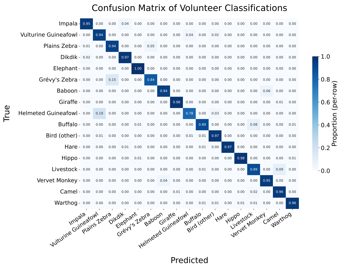
Figure S4: Confusion matrix for human volunteers for the Prickly Pear dataset. Matrix rows represent true test set labels, while matrix columns represent volunteer predictions. Species are sorted by the number of (true) occurrences in the test set.
