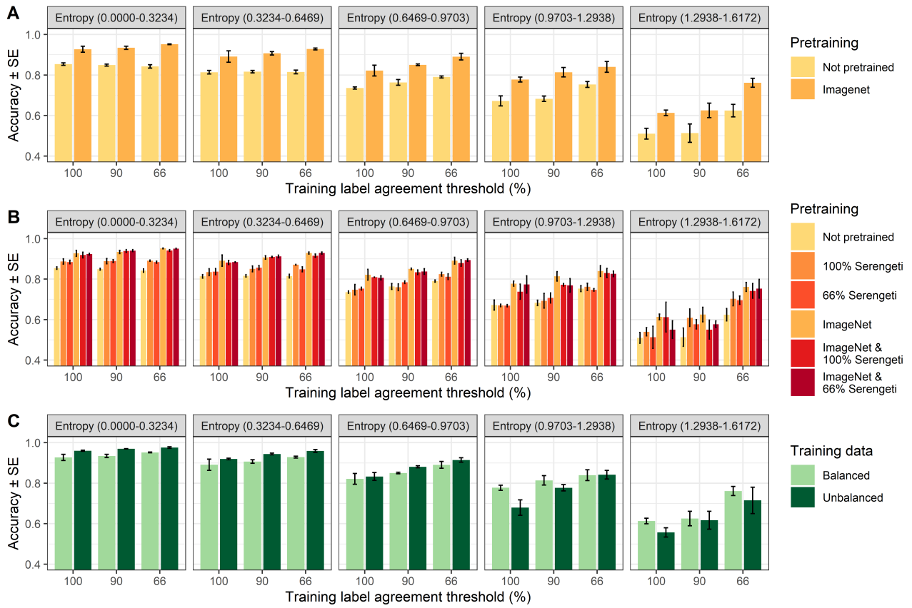
Figure 2: Test accuracy (proportion of correct classifications; mean \pm standard error) for the Prickly Pear Project Kenya dataset under different volunteer agreement thresholds (%) for label acceptance, for models which were A) either not pre-trained, or pre-trained on ImageNet, B) additionally pre-trained on Snapshot Serengeti images with either 100% or 66% volunteer agreement thresholds, and C) trained using a balanced or unbalanced dataset. Panels represent different levels of image difficulty as measured by the Shannon entropy of the volunteer classifications; higher entropy values (towards right) indicate more volunteer disagreement, and hence more difficult images. Sample sizes for entropy bins are (left to right) 6725, 2181, 1003, 255, and 92 images. Five images with entropy > 1.5395 were excluded.
