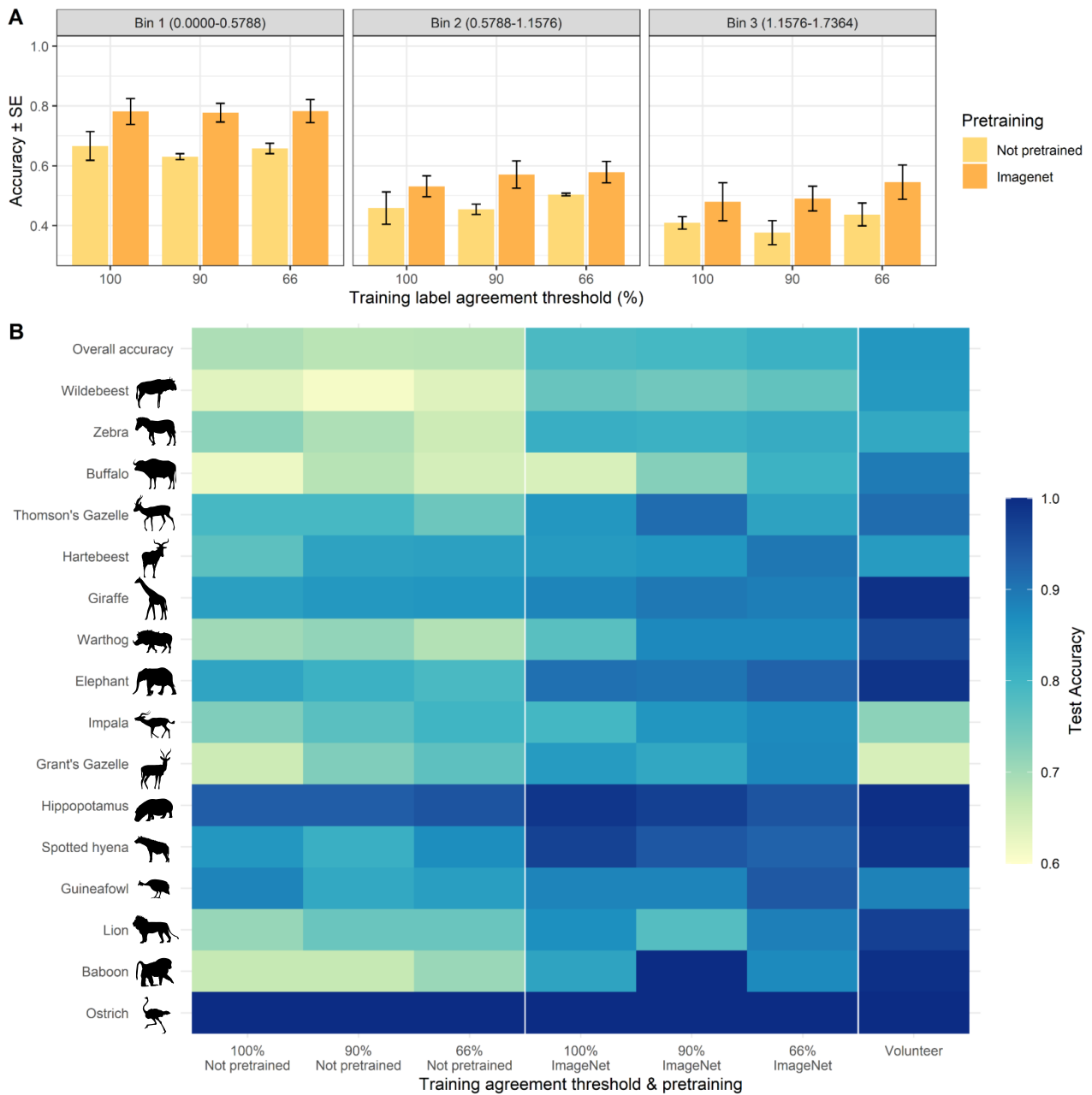
Figure S1: Results for the Snapshot Serengeti test set, for models trained under different volunteer agreement thresholds (%) for label acceptance and either not pre-trained or pre-trained on ImageNet. A) Test accuracy (proportion of correct classifications; mean \pm standard error) across different levels of image difficulty as measured by the Shannon entropy of the volunteer classifications; higher entropy values (towards right) indicate more volunteer disagreement, and hence more difficult images. Sample sizes for entropy bins are (left to right) 2635, 298, 49. Three images with entropy > 1.7364 were excluded. B) Species-level classification accuracy (true positive rate). Volunteer accuracy is also displayed on the rightmost column. The top row displays overall test accuracy across all species. Species test set sample sizes are: wildebeest (1356), zebra (782), buffalo (164), Thomson's gazelle (151), hartebeest (97), giraffe (79), warthog (75), elephant (73), impala (72), Grant's gazelle (46), hippopotamus (25), spotted hyena (23), guineafowl (17), lion (15), baboon (8), ostrich (2).
