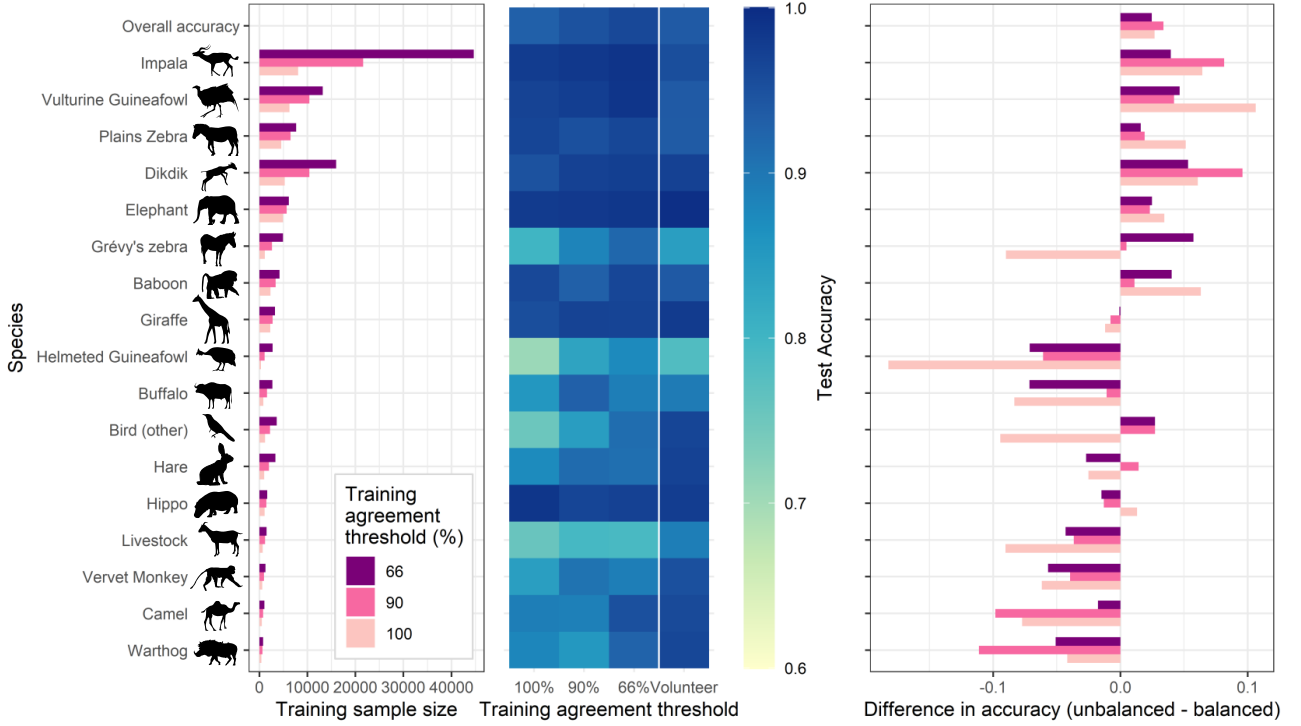
Figure 5: Species-specific classification accuracies for the Prickly Pear Project Kenya dataset, using unbalanced training data. Left: Number of images per species in training set set under different training label agreement thresholds ( \geq 66\% , 90\% , 100\% ). Centre: Test accuracy (true positive rate) for different agreement thresholds and human volunteers. The top row displays overall test accuracy across all species. Right: Difference in test accuracy between models trained on unbalanced and balanced data; positive values indicate better performance when trained on unbalanced data. Separate bars for each species represent different label agreement thresholds. Species are ordered by frequency of occurrence in the test set, from most (top) to least common (bottom).
