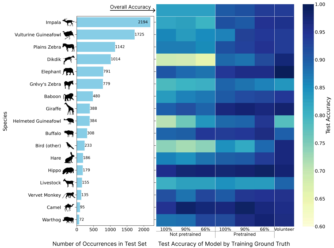
Figure 4: Species-level classification accuracy for the Prickly Pear Project Kenya Dataset, trained on a balanced dataset. Left: Number of images per species in test set. Right: Test accuracy (true positive rate). Models were either trained from random initialization or pre-trained, and then trained on data with varying agreement thresholds ( \geq 66\% , 90\% , 100\% ) for label acceptance. Volunteer accuracy is also displayed on the rightmost column. The top row displays overall test accuracy across all species.
