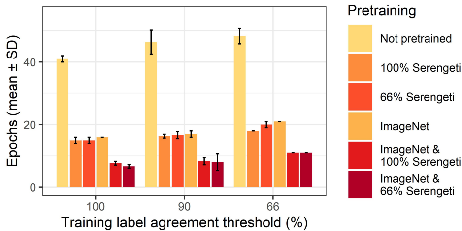
Figure 3: Number of epochs (mean \pm standard deviation) taken to reach 0.97 training accuracy, for models trained with different label agreement thresholds (%) and pre-training treatments.
