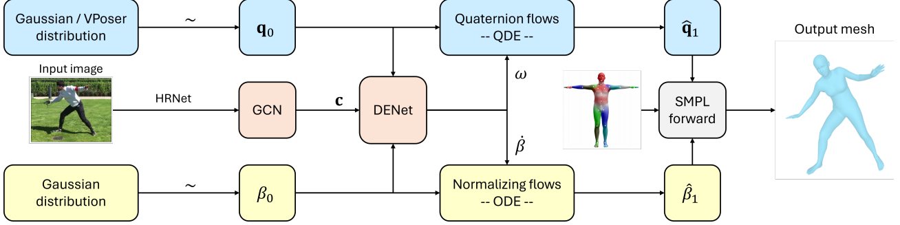
Figure 2. Pipeline of CQF-HMR. The method consists of two differential equations: an QDE for the quaternion flows and an ODE for the shape normalizing flows. The initial pose \mathbf{q}_0 and shape \beta_0 are sampled from source distributions, i.e. Gaussian distribution, while GCN encodes the 2D heatmaps extracted by HRNet to obtain the lifting condition \mathbf{c} . DENet estimates the angular velocity \omega and shape shifting rate \dot{\beta} for the predictions of quaternion pose \hat{\mathbf{q}}_1 and shape \hat{\beta}_1 under the S^3 constraint with OT transports. The 3D mesh is obtained by passing the predicted pose and shape to the SMPL transformation layer. The pipeline is executed in parallel for multiple hypotheses.
