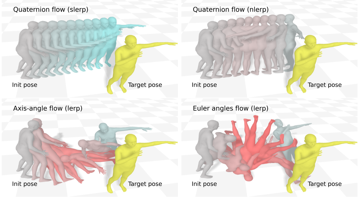
Figure 3. The comparison between the OT flows of the 3D rotations: quaternion with slerp , quaternion with nlerp (normalized lerp ), Euler angles with lerp , and Axis-angle with lerp . The yellow mesh is the ground-truth pose from the Human3.6M test split. Blue indicates low MPJPE, while red indicates high MPJPE. The init pose is sampled from the VPoser distribution [32], and the normalizing flow direction is from left to right. The trajectories are obtained by solving the ODEs with their respective OT derivatives.
