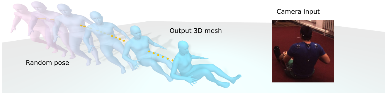
Figure 1. Conditioned on a 2D input estimated from a single image, our CQF-HMR maps a randomly sampled 3D human pose to a plausible one using the continuous normalizing flows under the quaternion constraint. Unlike other 3D rotation representations, quaternion flows provide smoother generation trajectories, leading to a more plausible 3D human mesh recovery.
