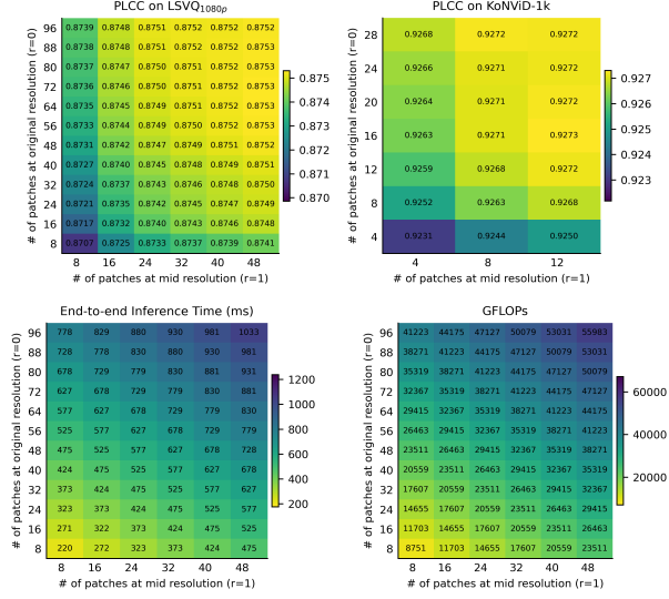
Figure 2. PLCC on LSVQ 1080p and KoNViD-1k, together with end-to-end inference time and GFLOPs, as a function of the number of ST patches at scales r = 0, 1 , with 6 patches fixed at the coarsest scale r = 2 .
