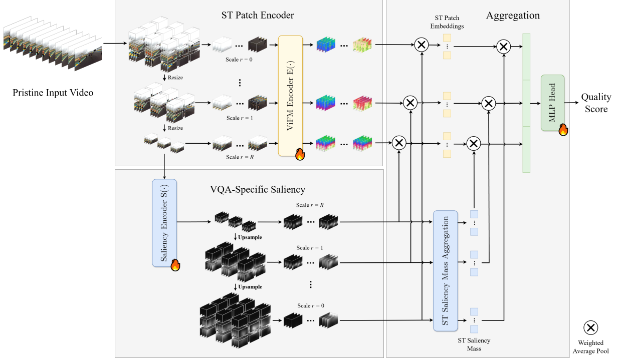
Figure 1. HFVQA pipeline. Multi-scale ST patches are sampled, with VQA-specific saliency predicted by S(\cdot) at the coarsest scale ( r = R ). Independently encoded patches are aggregated using the resulting saliency volumes.
