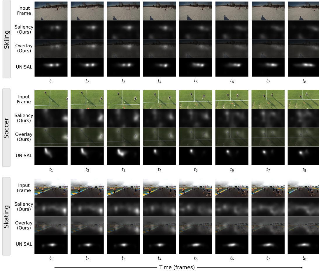
Figure 3. Consecutive video frames (top), learned VQA-specific saliency maps (second), overlays (third), and comparison with UNISAL (bottom). Best viewed zoomed in.
