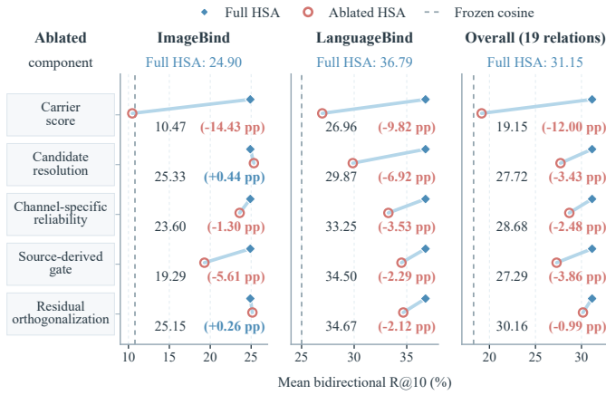
Fig. 9. Complete Component Ablation of the HSA Readout. Mean bidirectional Recall@10 for full HSA and five matched single-component variants on ImageBind, LanguageBind, and all nineteen relations.
