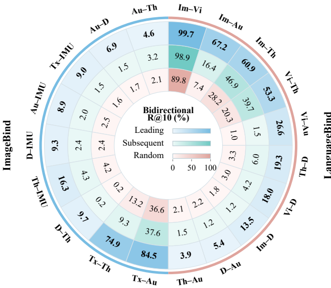
Fig. 5. Spectral Carrier Localization in Complete HSA. From outer to inner, the three heatmap rings report bidirectional Recall@10 (%) for leading, subsequent, and random paired directions. Carrier counts and assigned reliability spectra are matched within each relation. Results for random directions are averaged over five seeds.
