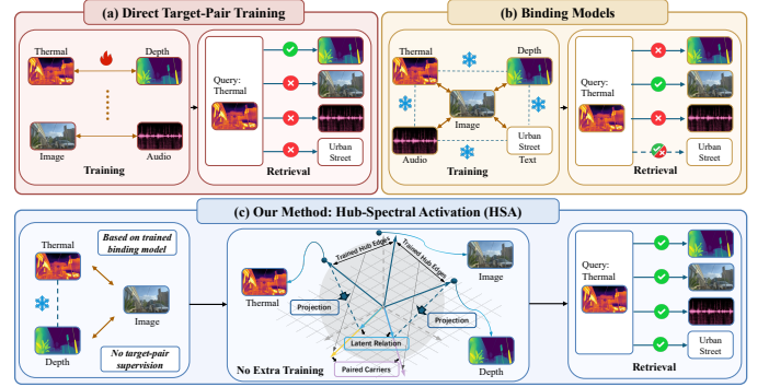
Fig. 1. From Multimodal Training to Hub-Spectral Activation. (a) Target-pair training learns one relation from paired data. (b) Hub-based binding reduces pairwise supervision but leaves held-out retrieval uneven. (c) HSA reads the relation supported by two trained hub connections and produces retrieval rankings. HSA improves held-out retrieval in closed form, with frozen encoders and without positive target-pair examples or gradient optimization.
