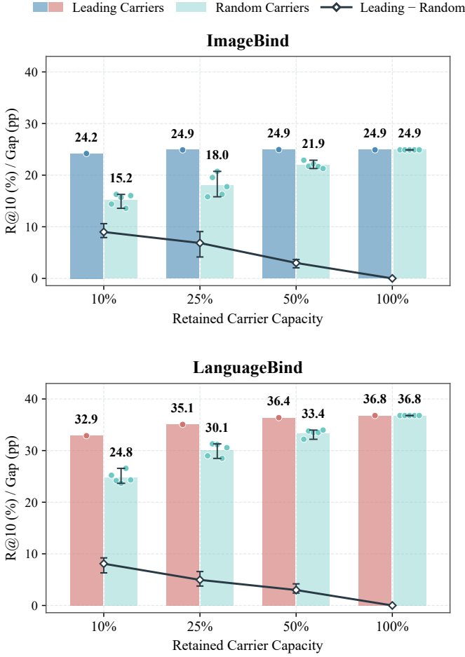
Fig. 7. Backbone-Level Carrier Accumulation in HSA. Bars show mean bidirectional Recall@10 for leading and random carriers; circles mark the leading result and five seed-specific random means. Diamonds show leading-minus-random gaps in percentage points; error bars span the seed range.
