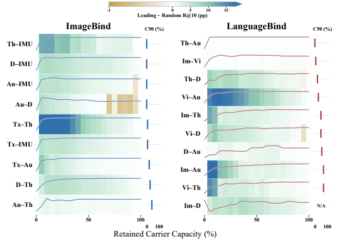
Fig. 6. Relation-Wise Carrier Capacity in HSA. Curves show retrieval performance as progressively more leading carriers are retained. Background colors indicate Recall@10 differences from equal-count random carrier subsets, in percentage points. C90 denotes the minimum retained capacity that sustains at least 90% of the full-carrier gain over the zero-carrier baseline; N/A indicates a nonpositive full-carrier gain.
