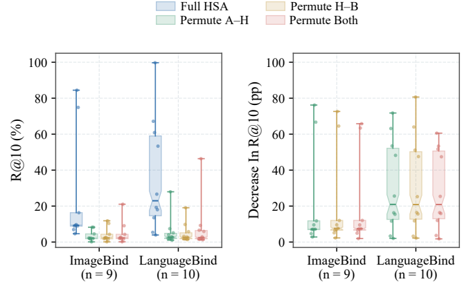
Fig. 3. Hub-Edge Correspondence in Complete HSA. Left: Recall@10 under intact correspondence and three permutation controls. Right: paired decreases in percentage points. Each dot represents a relation; permutation results average five refits. Boxes span the interquartile range, schematic notches mark medians, and whiskers span observed extrema.
