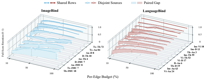
Fig. 4. Source-Sample Scaling under Shared and Disjoint Estimation. Bidirectional Recall@10 for each relation across ten nested per-edge budgets, normalized by the shared-row result at the full budget. Filled and hollow markers denote shared-row and disjoint-source estimation, respectively; shaded ribbons show their paired gaps. Numbers beside the relation labels report the shared-row Recall@10 (%) at the full budget.
