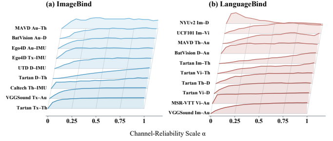
Fig. 8. Reliability-Controlled Spectral Activation in HSA. Each curve shows the change in bidirectional Recall@10 relative to \alpha = 0 , normalized by the maximum observed increase for that relation across 21 channel-reliability scales in [0, 1] . Panels (a) and (b) show results for ImageBind and LanguageBind, respectively.
