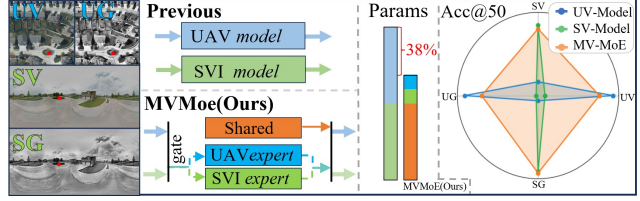
Figure 2. Comparison of the proposed MV-MoE and independent models. MV-MoE shares one encoder and two lightweight experts (UAV, SVI) for four input variants (UAV Vis, UAV Gray, SVI Vis, SVI Gray), reducing parameters by 38% while maintaining Acc@50 (%).
