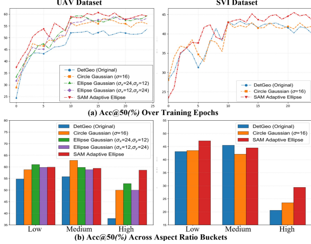
Figure 8. ESAM-Prior ablation results on UAV and SVI datasets. (a) Validation Acc@50 (%) over training epochs. (b) Acc@50 (%) across object aspect ratio buckets partitioned into Low, Medium and High groups.
