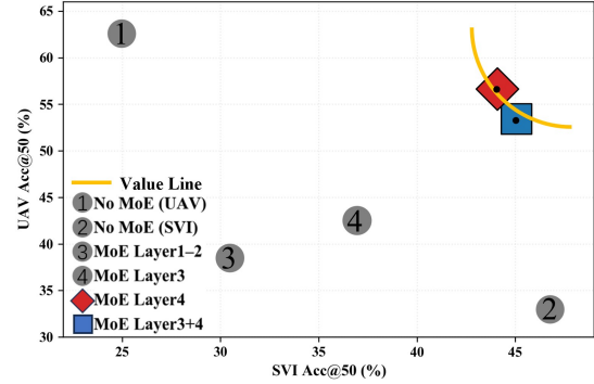
Figure 7. Cross-dataset localization accuracy distribution on UAV and SVI scenes. The yellow value line denotes the Pareto trade-off boundary, and points above the line achieve superior overall performance.
