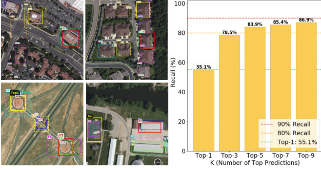
Figure 4. Recall@K reveals that the ground-truth box often appears among top candidates but is not ranked first.
