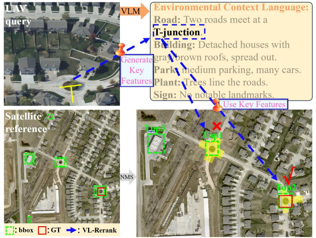
Figure 1. Illustration of the VL-Rerank framework. A VLM generates environmental context (e.g., road topology) from query images. These descriptions rerank satellite candidates, filtering out visually similar but contextually mismatched bounding boxes and identifying the correct target.
