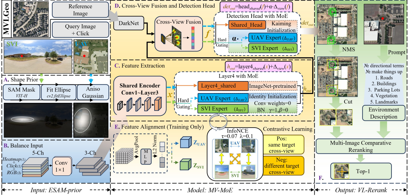
Figure 3. Schematic diagram of the MVLGeo network architecture. (A) Input-guided features are generated using SAM and shape priors. (B) Balancing heterogeneous input channels. (C–D) Using a Mixture-of-Experts (MoE) architecture with hard gating to perform cross-view feature extraction, fusion, and detection from UAV and SVI perspectives. (E) Aligning cross-view features during the training phase via InfoNCE contrastive learning. (F) Performing multi-image comparison and reranking by combining environmental semantic descriptions and image cropping to output the Top-1 matching result.
