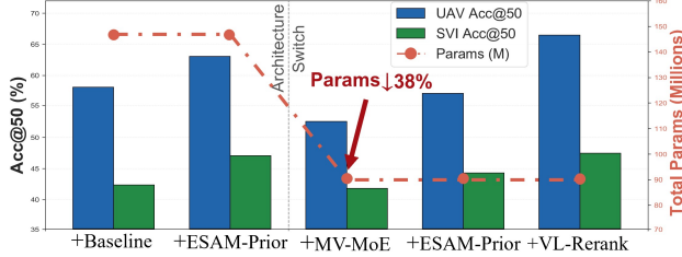
Figure 6. Contributions of each component to the UAV and SVI test sets, and corresponding parameter relationships.
