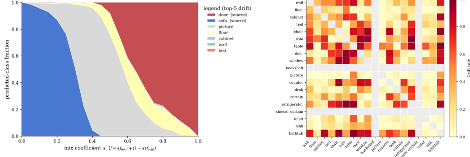
Figure 2: Semantic drift from linear interpolation of CLIP features. Left: mixing the source features of door and sofa as f = \alpha f_{\text{door}} + (1 - \alpha) f_{\text{sofa}} . The predicted class drifts to unrelated categories (e.g. picture , floor ) for \alpha \in [0.3, 0.7] , with neither source class dominating in this regime. Right: pairwise drift rate at \alpha=0.5 across the 19 ScanNet classes used in our protocol; the overall drift rate is 33.6%.
