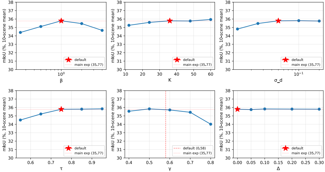
Figure 4: Hyperparameter sensitivity on ScanNet (10-scene mean, 19 classes). Each subplot shows mIoU as a function of one hyperparameter, with the others fixed at their defaults. The default value is marked by a red star (or a dashed vertical line when the default does not coincide with the swept points), and the dotted red line indicates the main-experiment mIoU (35.77). Across all six hyperparameters, mIoU stays within [34.0, 35.95] , demonstrating that NormLift is robust to reasonable hyperparameter choices.
