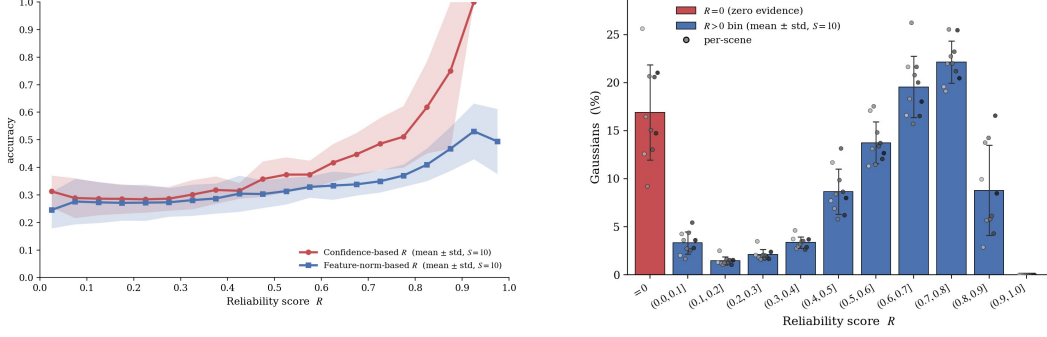
Figure 5: Reliability calibration and distribution on ScanNet. Left: the proposed reliability score R aligns more monotonically with downstream accuracy than the feature-norm-based score, showing the benefit of effective multi-view calibration. Right: Gaussian distribution over reliability intervals, with zero-evidence Gaussians ( R = 0 ) shown in red and nonzero bins shown in blue. The results indicate that R provides an informative per-Gaussian signal for identifying unreliable primitives and guiding refinement.
