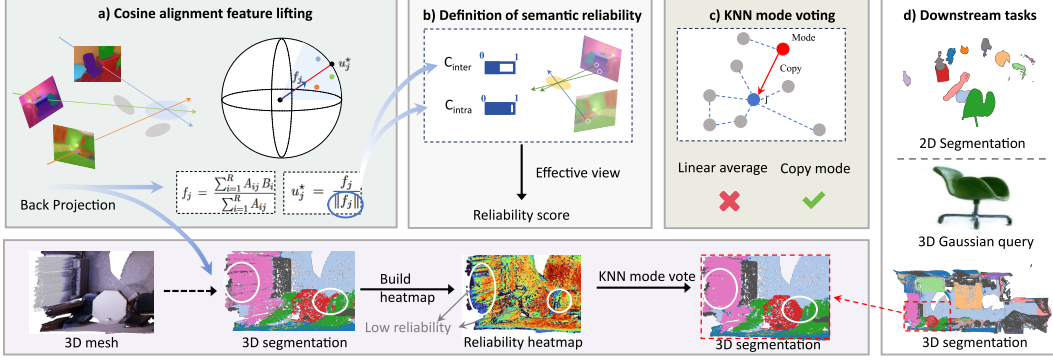
Figure 1: Method overview of NormLift. Top: a) Per-Gaussian features are lifted via cosine alignment on the CLIP sphere, giving the closed-form u_j^* = f_j / \|f_j\| . b) The norm \|f_j\| factors into intra- and inter-view consistency, calibrated to the reliability score R(j) by effective view support. c) KNN mode voting copies the most-supported neighbor’s feature, avoiding the blur of linear averaging. d) NormLift supports 2D and 3D downstream tasks. Bottom: a visualization of the 3D segmentation pipeline. The framework is training-free and operates entirely at the per-Gaussian level.
