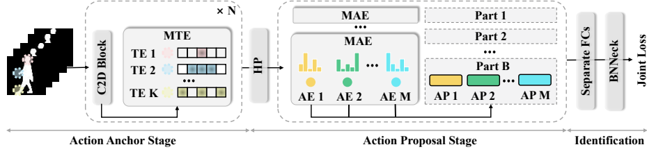
Fig. 3: The overview of GaitMoE. Best viewed in colors, the input sequence is firstly extracted to frame-level features by C2D Block ( e.g. , 2D CNNs or a residual block), and Mixture of Temporal Experts (MTE) dispatch temporal experts (TE) with different temporal bounding boxes to the corresponding channel segments, forming action anchors. After horizontal partitioning (HP), Mixture of Action Experts (MAE) is independent for each part-level feature. For each channel segment, one action expert (AE) integrates similar action anchors along the temporal dimension by weighted sum operation, forming one action proposal. Finally, The concatenated action proposals as part features for identification.
