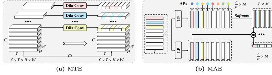
Fig. 4: (a) Mixture of Temporal Experts. Dila Conv (DC) represents Dilated Convolution, predefining action anchors with different dilated ratios. (b) Mixture of Action Experts. LP denotes the linear projection. Similar action anchors adaptively integrate into action proposals.
