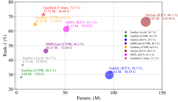
Fig. 7: The model comparisons on accuracy and efficiency. Rank-1 (%), Param. (M) and FLOPs. (G) on Gait3D.
