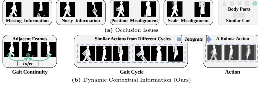
Fig. 1: (a) The main four occlusion issues in gait recognition. (b) The dynamic contextual information within a gait sequence can infer and integrate occlusion information.
