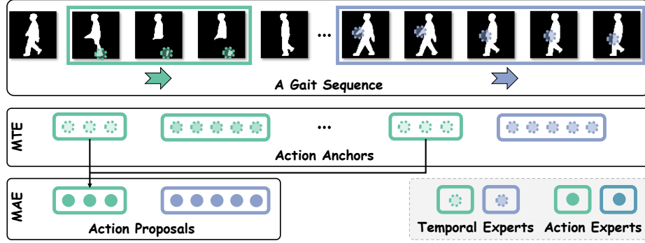
Fig. 2: Action composition. Each temporal expert focuses on one body region with individual temporal size, constructing action anchors. Each action expert integrates similar action anchors from different gait cycles, constructing one action proposal.
