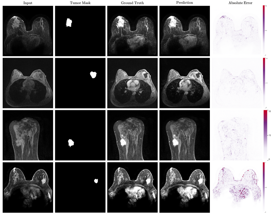
Fig. 3. Qualitative results of the selected model (LoRA rank/ \alpha = 64/64 , \text{MHA}_{\max} = 25 , \lambda_{\text{tumor}} = 0.25 , \lambda_{\text{stable}} = 0.1 ). The predictions preserve the main anatomical structure and produce spatially aligned enhancement patterns in the shown examples. Residual errors are visualized with independently scaled error maps for each case.
