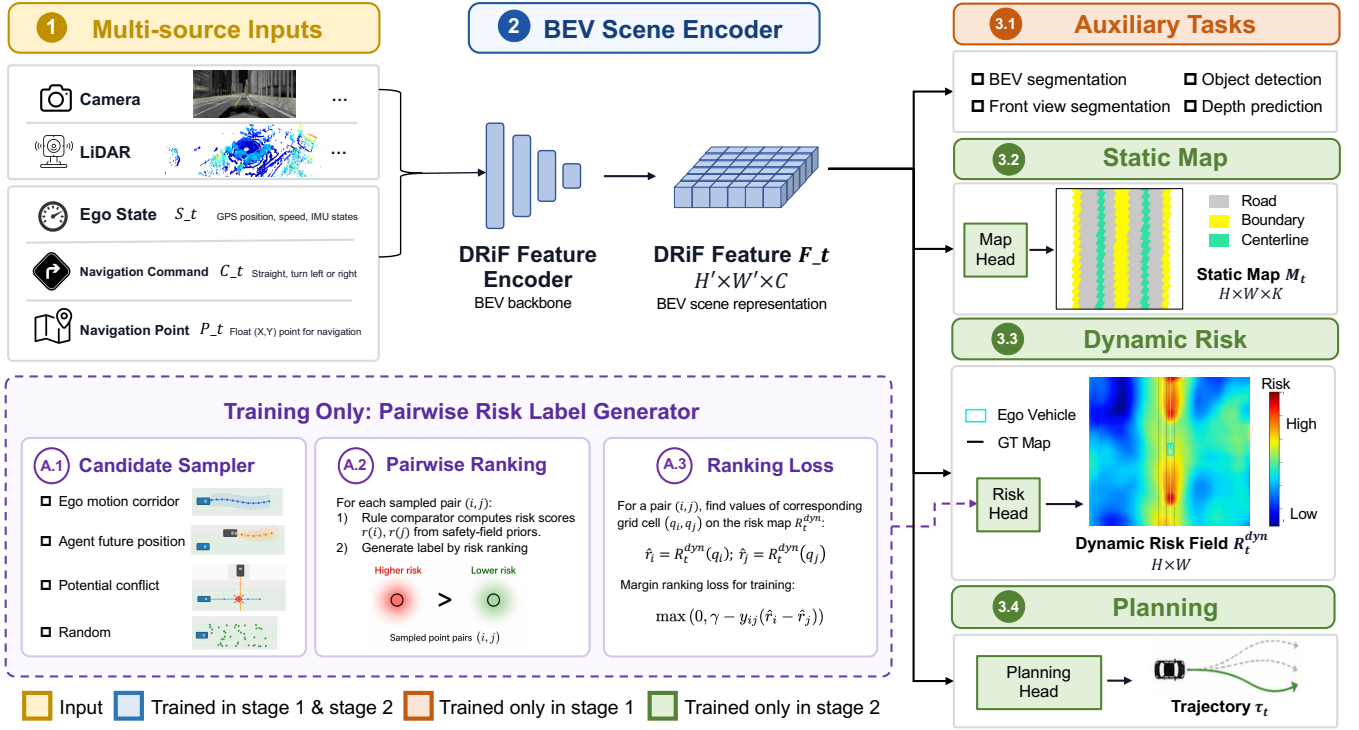
Fig. 2: Overview of DRiF. DRiF encodes multi-source driving inputs into a shared BEV feature F_t for auxiliary perception, static map segmentation, dynamic risk prediction, and trajectory planning. The model is trained in two stages. Stage 1 uses auxiliary tasks to pretrain the encoder with directly observable scene knowledge (e.g., object states). Stage 2 removes the auxiliary perception branch and jointly trains the static map, dynamic risk, and planning branches. The dynamic risk head is supervised by pairwise risk labels generated from rule-based safety priors, while the static map head maintains the model's understanding of static surroundings.
