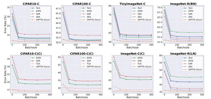
Fig. 2. Sensitivity analysis of batch size, where C indicates the CTTA.
