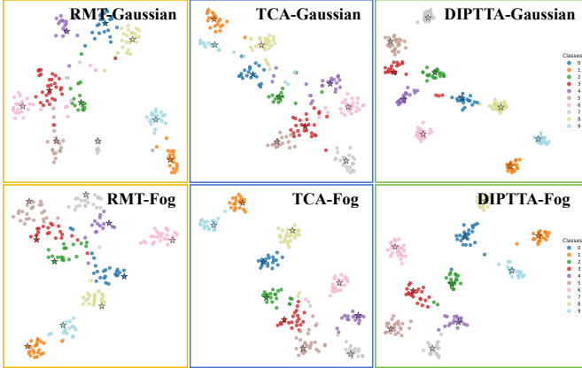
Fig. 4. Visualization of t-SNE for two methods and our proposed DIPTTA on CIFAR10-C (TTA Scenarios). We select a random batch of features from the Gaussian and Fog domains for comparative visualization.
