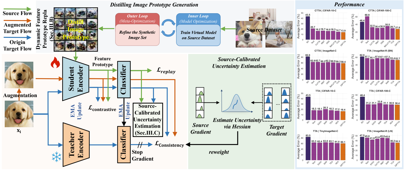
Fig. 1. Overall framework of our proposed DIPTTA. The top part visualizes the Distilling Image Prototype (DIP) module, which generates high-fidelity synthetic prototypes via a two-loop distillation strategy. The bottom part depicts the core online adaptation pipeline, where a student model is continuously updated with the guidance of a teacher model. Specifically, a source-calibrated uncertainty estimation and reweighting mechanism is embedded to dynamically calibrate the gradient contribution from target data, effectively mitigating distribution shift issues in open-world adaptation scenarios.
