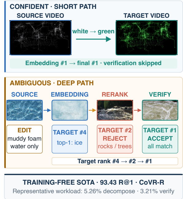
Figure 1. Two different pipeline paths through our confidence-gated cascade. A confident case skips heavy verification stages, while an ambiguous case utilizes reranking and strict verification to correct the top prediction after coarse retrieval favours a distractor. The footer summarizes complete accuracy and stage-wise workload spread on the CoVR-R dataset.
