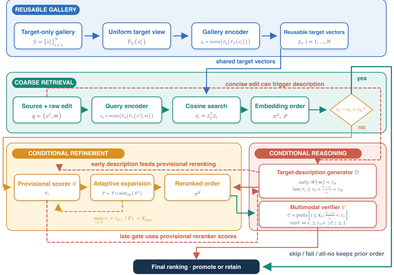
Figure 2. Overview of the training-free retrieval cascade. Reusable gallery encoding supports global search, while confidence gates route only uncertain queries through bounded candidate scoring, target-description generation, and strict multimodal verification. Skipped or unresolved conditional stages retain the preceding valid ranking.
