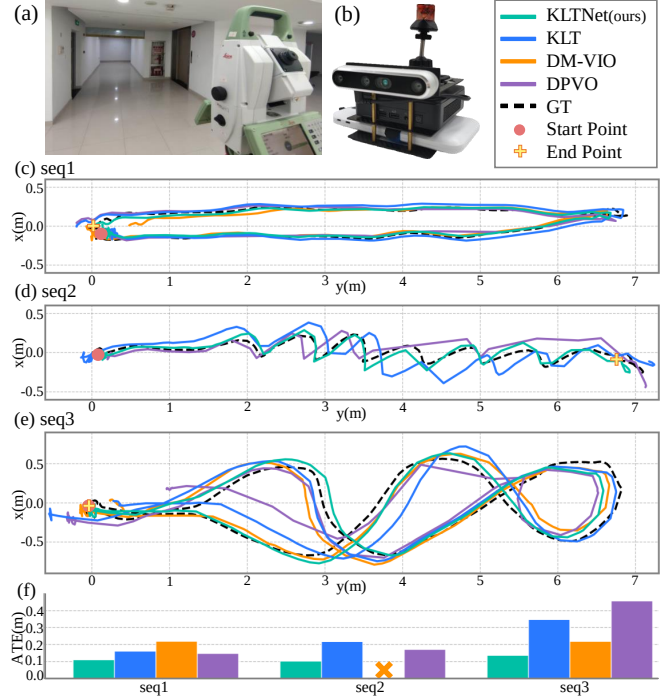
Fig. 4. VIO performance on a self-collected low-texture dataset. (a) A view of the challenging low-texture environment. (b) The handheld data acquisition platform. (c)–(e) Estimated trajectories for KLTNet-VINS-Mono compared against KLT-VINS-Mono, DM-VIO, and DPVO. (f) Absolute Trajectory Error (ATE) in meters. Note that DM-VIO failed to track in seq2.
