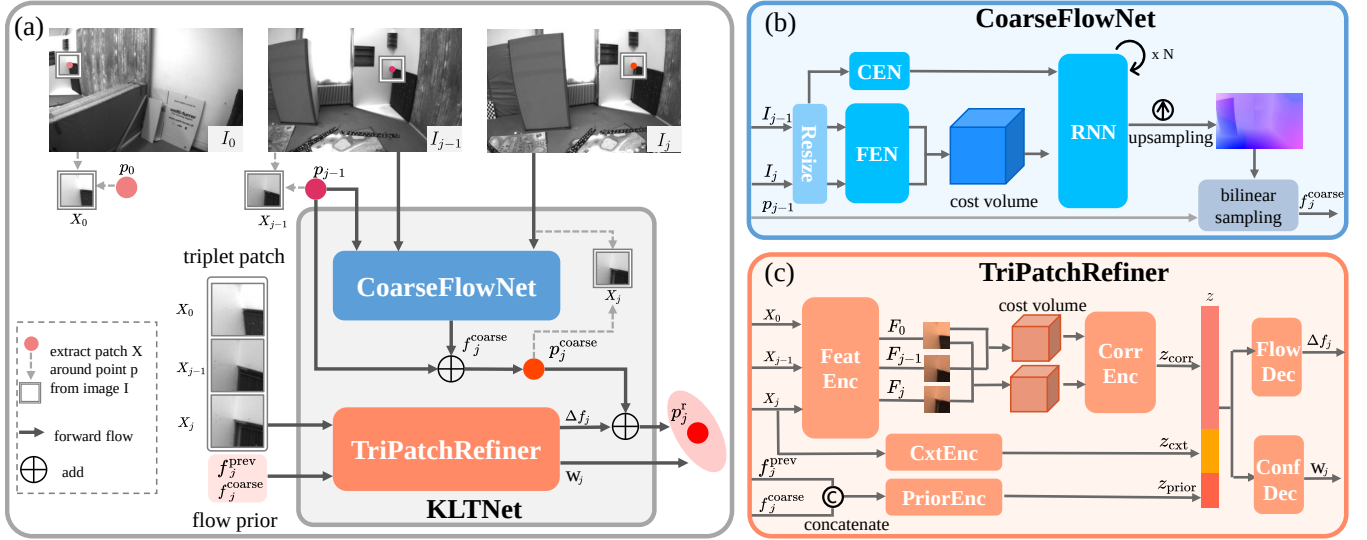
Fig. 2. (a) Overview of the KLTNet tracker for sparse feature tracking, illustrated with a single point for clarity. Given a feature p_0 with its reference patch X_0 , and its tracked position p_{j-1} with corresponding patch X_{j-1} , CoarseFlowNet first estimates a coarse flow f_j^{\text{coarse}} between previous frame I_{j-1} and the current frame I_j to predict an initial position p_j^{\text{coarse}} . The TriPatchRefiner then processes the triplet image patch (X_0, X_{j-1}, X_j) , where X_j is extracted around p_j^{\text{coarse}} , along with flow priors to regress a fine offset \Delta f_j and a confidence weight matrix W_j . The final tracked feature position is obtained by adding the refined offset to the initial prediction. (b) CoarseFlowNet architecture. It downscales input images, extracts features using FEN and CEN, constructs a cost volume, and iteratively refines flow using an RNN, followed by upsampling and bilinear sampling to get the coarse flow at the tracked point. (c) TriPatchRefiner architecture. It utilizes FeatEnc to encode triplet image patches. CorrEnc processes cost volumes constructed between patch features. CxtEnc encodes context from patch X_j , and PriorEnc encodes flow priors. The concatenated features are fed to FlowDec and ConfDec to predict offset and confidence weights, respectively.
