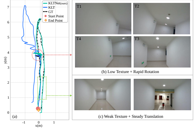
Fig. 1. Trajectory comparison in a low-texture environment using VINS-Mono with the classical KLT and the proposed KLTNet tracker. (a) KLTNet closely follows ground truth (GT), while classical KLT drifts under challenging scenarios. (b) During rapid rotation (T1–T4) in low-texture regions, KLT exhibits large drift (red dashed circle), but KLTNet remains stable. (c) In steady translation (green dashed box), both perform similarly, demonstrating that KLTNet performs comparably under moderate motion and remains robust when classical KLT degrades.
