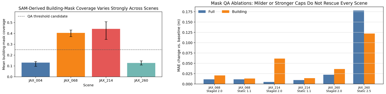
Figure 3: Mask-QA diagnostics. Coverage provides an interpretable prior-quality signal, and validation ablations complete the operating-policy decision.
