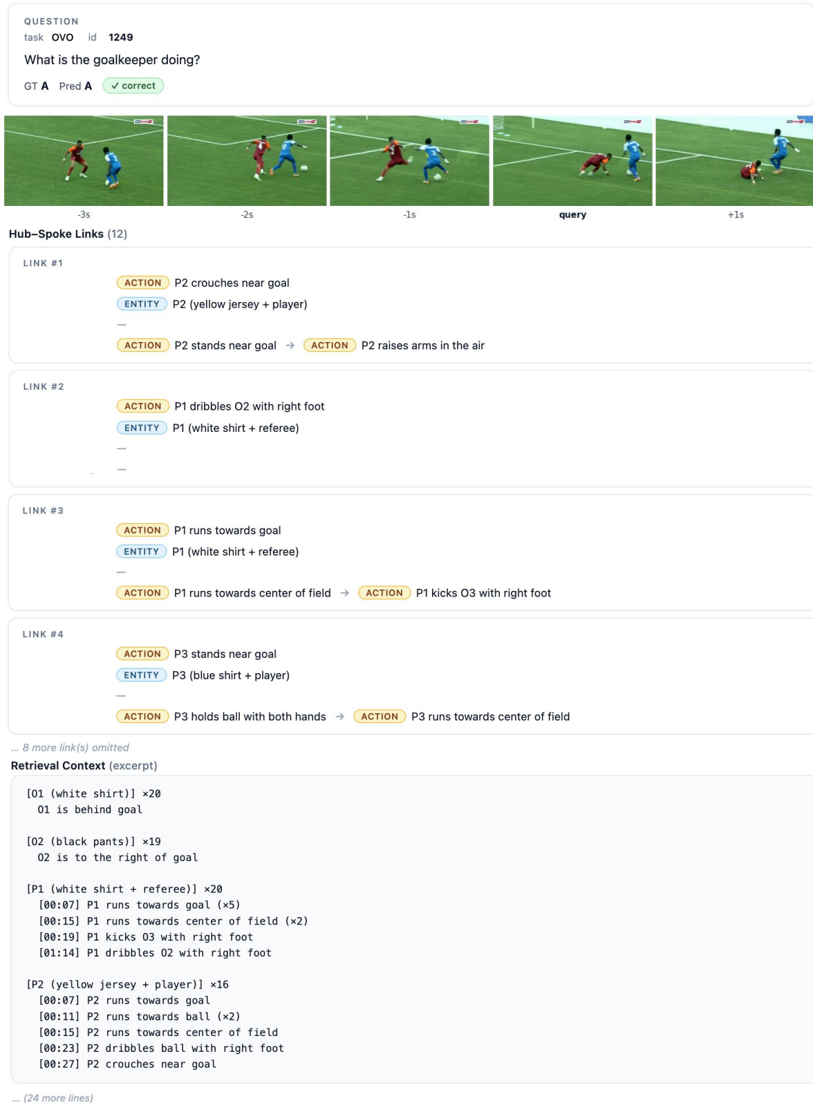
Figure D3: Visualization of hub-and-spoke memory details and the integrated retrieval context for the question from OVO-Bench.
