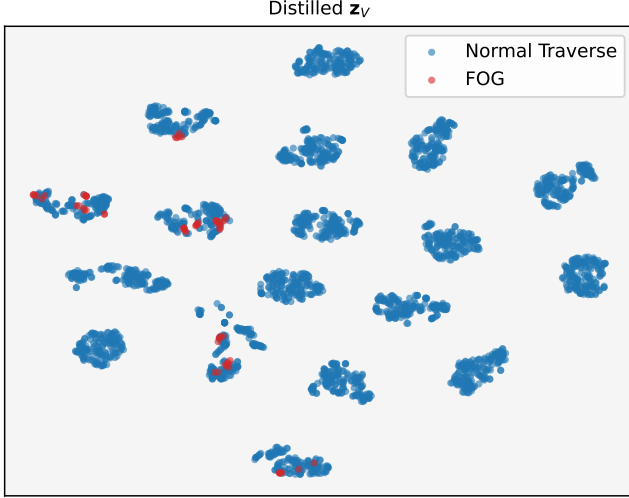
Fig. 3: Visual interpretation of t-SNE derived projections of the final z_V layer output distribution limits across inference test windows. Integrating objective inertial bounds (b) resolves severe sample overlap evident in unobstructed baseline estimations (a), minimising topological uncertainties during validation execution sequences.
