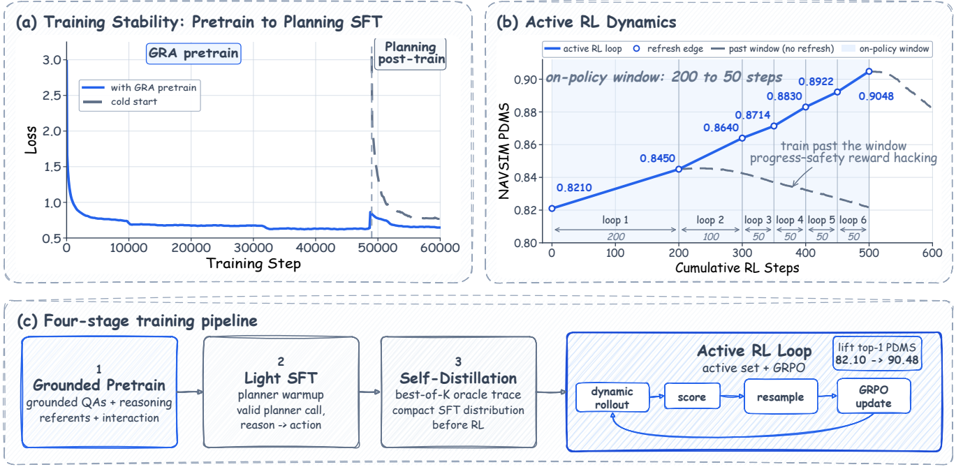
Fig. 4. Progressive training and Active RL dynamics of GRAVA. (a) Training loss with GRA pre-training and with planner training from a cold start (dashed). (b) Greedy NAVSIM PDMS across Active RL loops; shaded regions mark on-policy optimization windows. (c) Grounded pre-training, planner warm-up, verified self-distillation, and Active RL.
