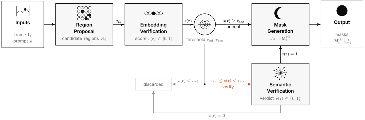
FIG. 1 ENEAS decision flow for semantic discovery. For every frame I_t and prompt p , region proposal yields candidate regions \mathcal{R}_t ; embedding verification scores each candidate with s(\mathbf{r}) . Candidates above \tau_{\text{acc}} are accepted directly and those below \tau_{\text{rej}} are discarded; only the uncertainty interval in between is routed to semantic verification, where a vision-language model re-returns a verdict v(\mathbf{r}) . The accepted set \mathcal{A}_t is turned into one binary mask per instance by mask generation. Each stage is costlier than the previous one and sees fewer candidates.
