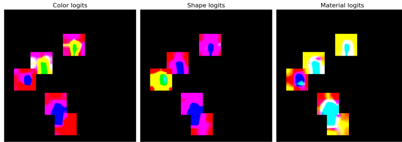
Fig. S2: Reconstructed model prediction for the color head (left), shape head (middle), and material head (right). Different colors indicate different predicted classes for the color, shape and material categories.
