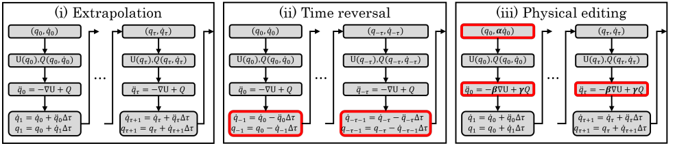
Figure 3: Overview of the physics manipulations. (i) Extrapolation: future states ( 0 < \tau ) are computed by forward integration. (ii) Time reversal: Past states ( \tau < 0 ) are recovered by backward integration using a negative time step -\Delta\tau . (iii) Counterfactual physics-based editing: Dynamic properties are manipulated by scaling the initial velocity ( \alpha ), learned potential ( \beta ), and time-independent non-conservative force ( \gamma ).
