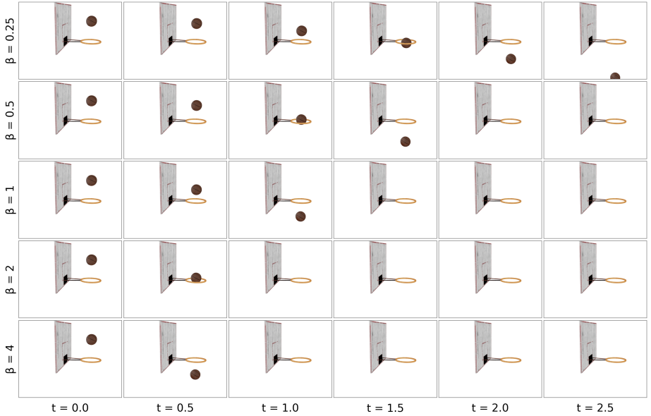
Figure 8: Inference-time counterfactual physics-based editing on the "Falling Ball" scene. The dynamics are systematically manipulated without retraining by rescaling the learned potential field ( U' = \beta \cdot U ). The baseline ( \beta = 1.0 ) reproduces the true observed trajectory. Decreasing \beta simulates a weakened gravitational environment, slowing the descent, while increasing \beta strengthens the effective gravity field. This predictable and continuous modulation exposes the learned U(q) as an explicitly editable physical property rather than an uninterpretable visual latent feature.
