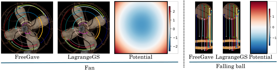
Figure 4: Learned trajectories of FreeGave and LagrangeGS with the potential U(q) for the "Fan" and "Falling Ball" scenes. While the rollouts of FreeGave exhibit erratic fluctuations, LagrangeGS ensures consistent trajectories satisfying Lagrangian mechanics. Without structural priors, U(q) captures the underlying physics: a rotationally symmetric potential for the Fan, and a uniform gravitational gradient for the Falling Ball.
