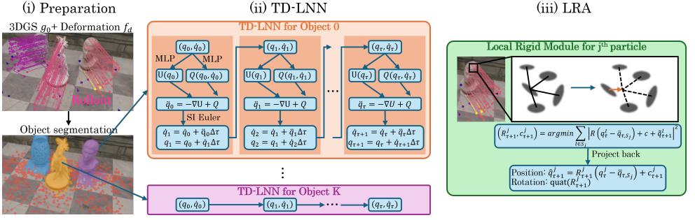
Figure 2: Overview of LagrangeGS. (i) Gaussian particles are partitioned into distinct objects via pre-trained model trajectory. (ii) TD-LNN computes per-particle accelerations \ddot{q} = -\nabla_q U + Q , combining the decoupled particle dynamics for avoiding intractable computation and the time-independent system for exact backward integration. (iii) To prevent geometric collapse, LRA binds the decoupled particles into locally rigid structures.
