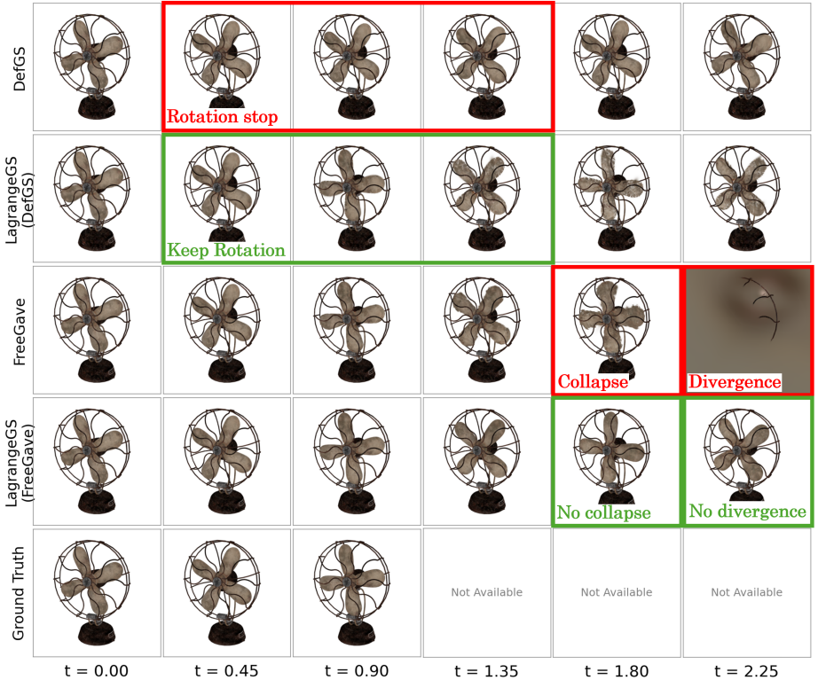
Figure 5: Extrapolation on the Fan scene. Training spans t = 0.0 – 0.75 . Upon entering extrapolation, DefGS instantly suffers from unnatural motion or complete stagnation, while FreeGave exhibits geometric drift at t = 1.80 and catastrophic volume divergence at t = 2.25 . Distilling both backbones via LagrangeGS (Ours) mitigates these artifacts, sustaining physically consistent and smooth rotation across the entire extended horizon.
