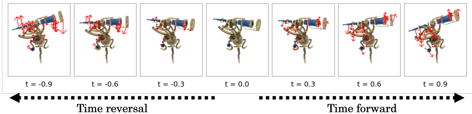
Figure 7: Time-reversal rollout on the "Telescope" scene via LagrangeGS. Past states ( t < 0 ) are recovered exactly by integrating the same trained TD-LNN backward with a negative time step -\Delta t , ensuring visual and structural consistency with forward rollouts ( t > 0 ). Red arrows denote per-particle velocity vectors; their exact directional inversion across t = 0 confirms that LagrangeGS captures genuine continuous mechanics rather than a learned animation shortcut.
