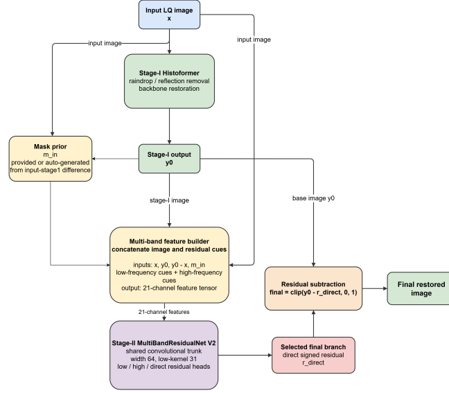
Fig. 9: The pipeline of the method proposed by Team ustc_pi_lab .
