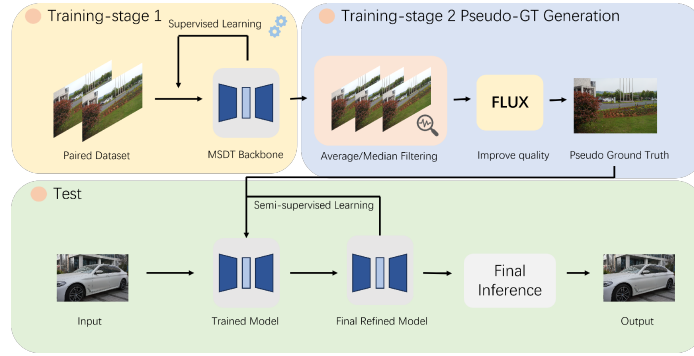
Fig. 8: The pipeline of the method proposed by Team AIIA-Lab.
