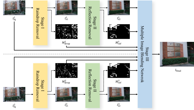
Fig. 3: The overall framework of Team GIST-IVL.
