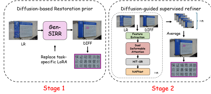
Fig. 2: The pipeline of the method proposed by Team tysl.
