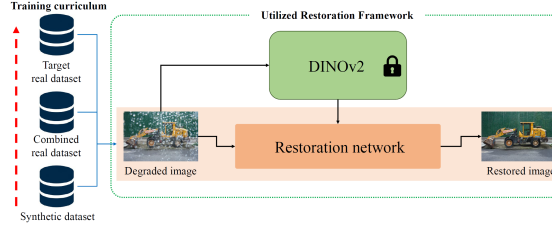
Fig. 6: The overall framework of Team SNU-ISPL.
