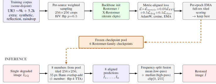
Fig. 7: The pipeline of the method proposed by Team the_last_token.
