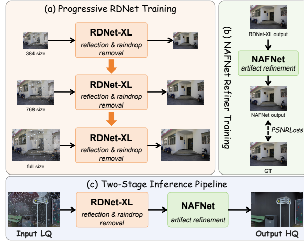
Fig. 1: The pipeline of the method proposed by Team Xedit Master .
