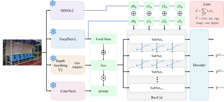
Fig. 5: The overall framework of Team ACVLAB.
