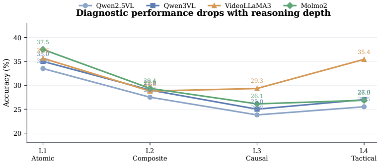
Figure 4: Level-wise zero-shot performance over single-choice and short-answer questions . The benchmark does not only test final answer correctness: it separates atomic recognition, composite understanding, causal reasoning, and tactical abstraction.
