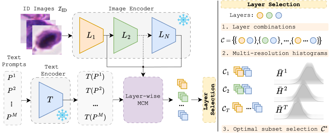
Fig. 2. Overview of the proposed intermediate-layer selection framework. Given in-distribution images I \in \mathcal{I}_{ID} and prompts \{P^1, \dots, P^M\} , the visual encoder outputs intermediate representations \{L_j(I)\}_{j=1}^N , which are projected into the shared image-text embedding space and scored via layer-wise MCM: S_{MCM}^{(j)}(I) . Candidate layer subsets C , always including the final layer N , are constructed, and their aggregated scores are collected across the in-distribution dataset to form the subset score distribution S_C . This distribution is evaluated via multi-resolution entropy \bar{H}(S_C) , and the optimal subset C^* minimizing aggregated entropy is selected for test-time inference.
