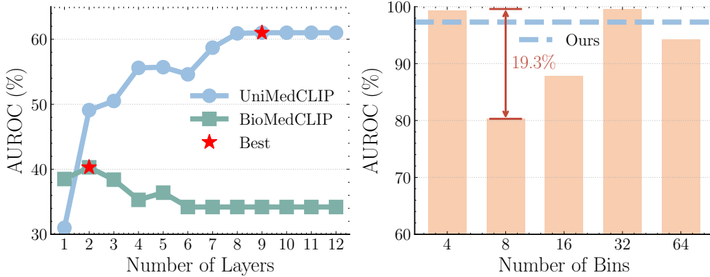
Fig. 3. Left: OOD performance on MIDOG (near) as a function of the number of aggregated intermediate layers. Right: Sensitivity analysis on OASIS (near) of single-resolution entropy-based layer selection across different histogram bin sizes, where performance varies by up to 19.3%. In contrast, our multi-resolution entropy estimation strategy achieves stable and near-optimal performance.
