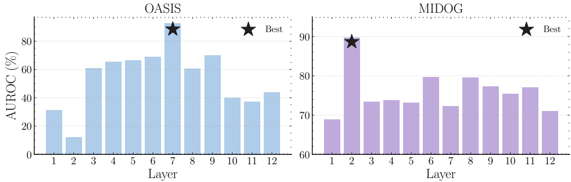
Fig. 1. Layer-wise zero-shot OOD detection performance (AUROC, %), using UniMedCLIP. Left: OASIS (brain MRI). Right: MIDOG (histopathology). Each bar corresponds to the OOD detection performance using Maximum Concept Matching (MCM) for the corresponding encoder layer, averaging for both near - and far -OOD shifts. The results demonstrate that the best layer depends on the dataset, i.e. , imaging modality. Notably, the final layer does not exhibit the best performance in either case.
